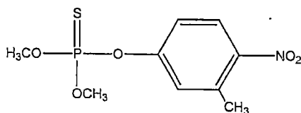
Fenitrothion
