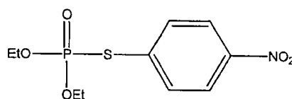
O,O'-diethyl-S-p-nitrophenylphosphorothioate
