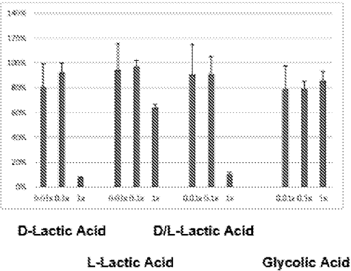
P. aeruginosa : compound added at time 0 h
