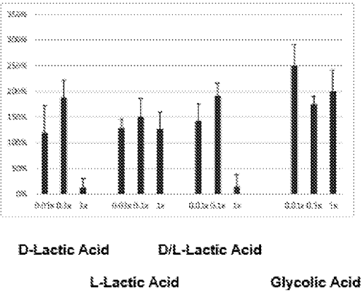
S. aureus : compound added at time 0 h
