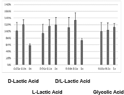
P. aeruginosa : compound added at time 24 h
