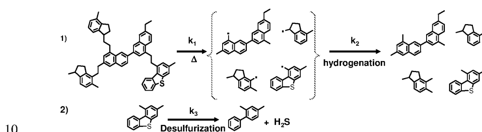
Scheme 2. Simplified reaction schemes summarizing main reactions occurring in the main hydroprocessing reactor.
