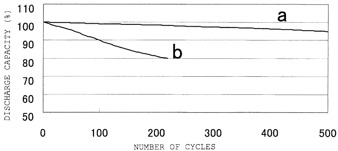
FIG. 1 CYCLE TEST AT 25°C
