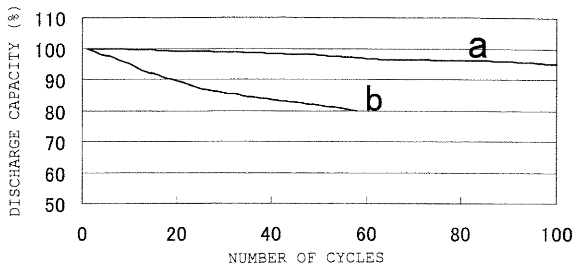
FIG. 3 CYCLE TEST AT -10^{\circ}\text{C}
