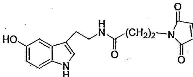
LBT3002 (4-(2,5-dioxo-2,5-dihydro-pyrrol-1-yl)-N-[2-(5-hydroxy-1 H -indol-3-yl)-ethyl]-butyramide)
