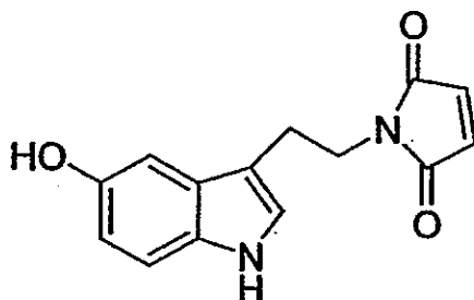
LBT3001 (1-[2-(5-hydroxy-1 H -indol-3-yl)-ethyl]-pyrrole-2,5-dione)
