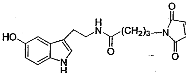
LBT3002 (4-(2,5-dioxo-2,5-dihydro-pyrrol-1-yl)-N-[2-(5-hydroxy-1 H -indol-3-yl)-ethyl]-butyramide)
