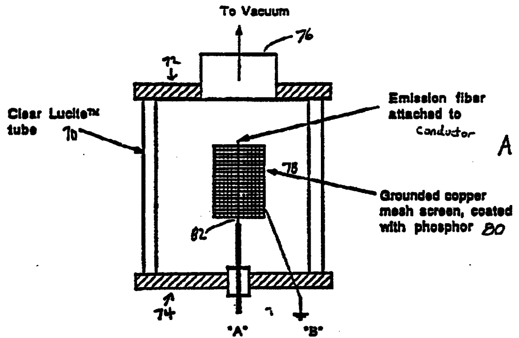
Fig. 5. FFEL Test Device
