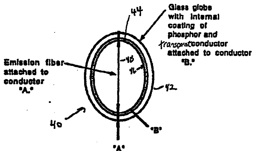
Fig. 3. 'Bulb' Shaped FFEL
