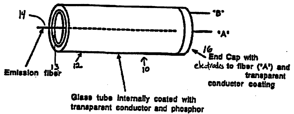
Fig. 1. Sectional View of Elongated Tube FFEL Device
