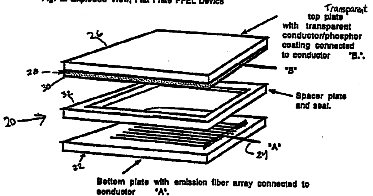
Fig. 2. Exploded View, Flat Plate FFEL Device
