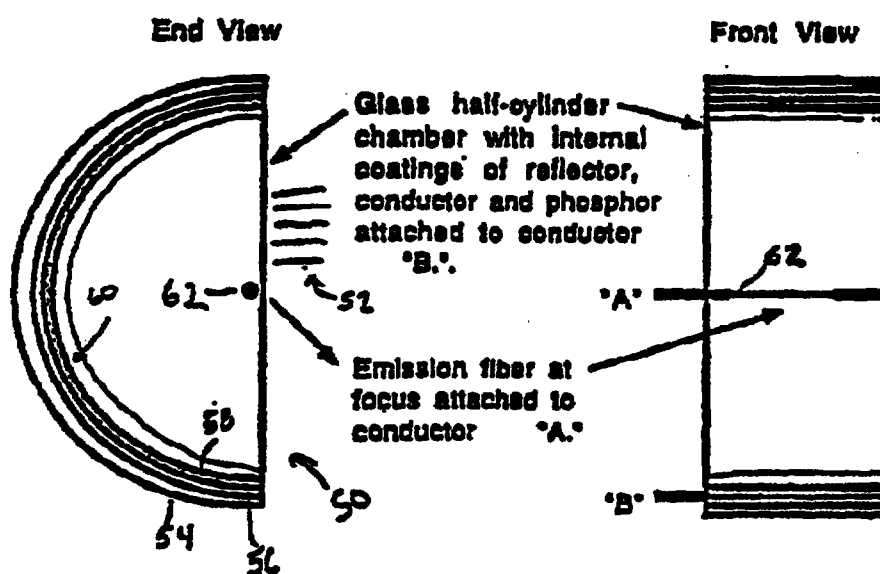
Fig. 4. FFEL Device for Producing Rectangular Beams
