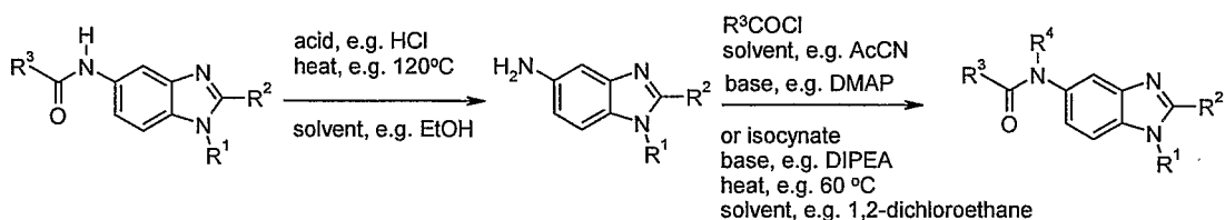
Scheme 2. (A synthetic route used for the synthesis of compounds including Examples 7 and 8)
