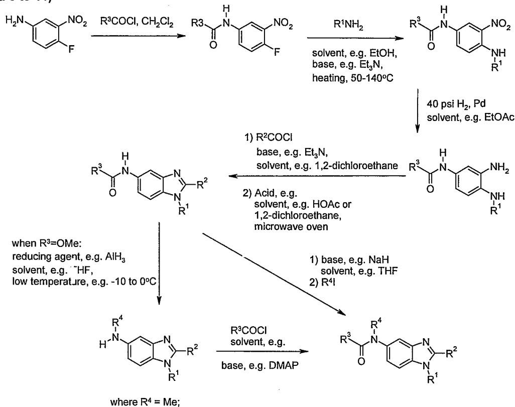
Scheme 1. (A synthetic route used for the synthesis of compounds including Examples 1 to 6 and 8 to 11)
