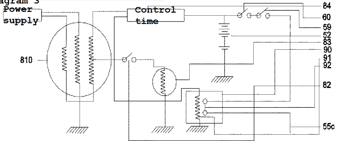
Circuit diagram 3
