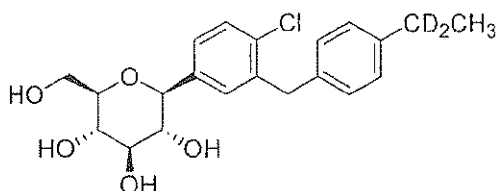
(2S,3R,4R,5S,6R)-2-(4-chloro-3-(4-(ethyl-1,1- d_2 )benzyl)phenyl)-6-(hydroxymethyl)tetrahydro-2H-pyran-3,4,5-triol;
