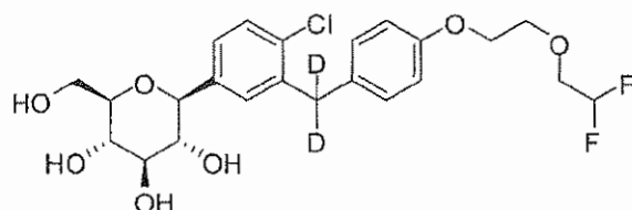
(2S,3R,4R,5S,6R)-2-(4-chloro-3-((4-(2-(2,2-difluoroethoxy)ethoxy)phenyl)methyl- d_2 )phenyl)-6-(hydroxymethyl)-tetrahydro-2H-pyran-3,4,5-triol;
