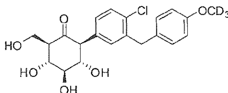
(2S,3S,4R,5R,6R)-2-(4-chloro-3-(4-(methoxy- d_3 )benzyl)phenyl)-3,4,5-trihydroxy-6-(hydroxymethyl)cyclohexanone
