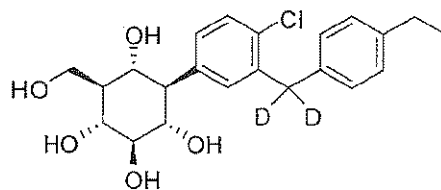
(1R,2R,3S,4R,5R,6S)-4-(4-chloro-3-((4-ethylphenyl)methyl- d_2 )phenyl)-6-(hydroxymethyl)cyclohexane-1,2,3,5-tetraol;
