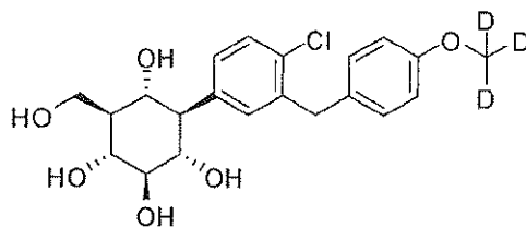
(1R,2R,3S,4R,5R,6S)-4-(4-chloro-3-(4-(methoxy- d_3 )benzyl)phenyl)-6-(hydroxymethyl)cyclohexane-1,2,3,5-tetraol;
