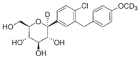
(2S,3R,4R,5S,6R)-2-(4-chloro-3-(4-(methoxy- d 3 )benzyl)phenyl)-6-(hydroxymethyl)tetrahydro-2 H -pyran-2- d -3,4,5-triol;
