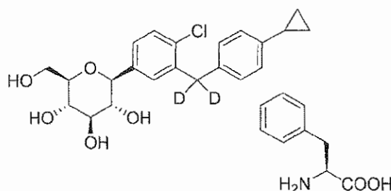
(2S,3R,4R,5S,6R)-2-(4-chloro-3-((4-cyclopropylphenyl)methyl- d_2 )phenyl)-6-(hydroxymethyl)tetrahydro-2H-pyran-3,4,5-triol, L-phenylalanine complex (1:1)
