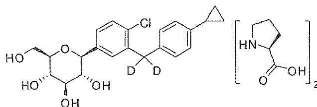
(2S,3R,4R,5S,6R)-2-(4-chloro-3-((4-cyclopropylphenyl)methyl- d 2 )phenyl)-6-(hydroxymethyl)tetrahydro-2H-pyran-3,4,5-triol, bis(L-proline) complex;
