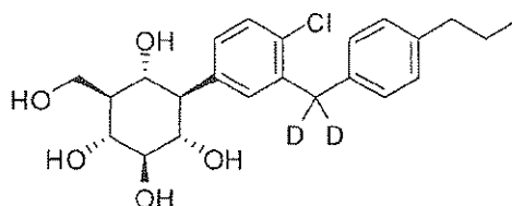
(1R,2R,3S,4R,5R,6S)-4-(4-chloro-3-((4-propylphenyl)methyl- d_2 )phenyl)-6-(hydroxymethyl)cyclohexane-1,2,3,5-tetraol;
