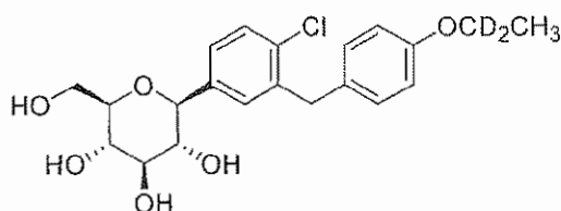
(2S,3R,4R,5S,6R)-2-(4-chloro-3-(4-(ethoxy-1,1- d_2 )benzyl)phenyl)-6-(hydroxymethyl)tetrahydro-2H-pyran-3,4,5-triol;
