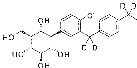
(1R,2R,3S,4R,5R,6S)-4-(4-chloro-3-((4-(ethyl-1,1- d 2 )phenyl)methyl- d 2 )phenyl)-6-(hydroxymethyl)cyclohexane-1,2,3,5-tetraol;
