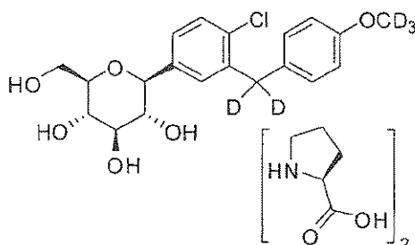
(2S,3R,4R,5S,6R)-2-(4-chloro-3-((4-(methoxy- d 3 )phenyl)methyl- d 2 )phenyl)-6-(hydroxymethyl)tetrahydro-2H-pyran-3,4,5-triol, bis(L-proline) complex;
