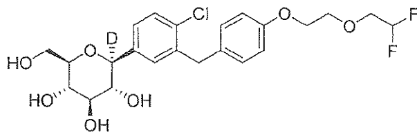
(2S,3R,4R,5S,6R)-2-(4-chloro-3-(4-(2-(2,2-difluoroethoxy)ethoxy)benzyl)phenyl)-6-(hydroxymethyl)tetrahydro-2H-pyran-2- d -3,4,5-triol;
