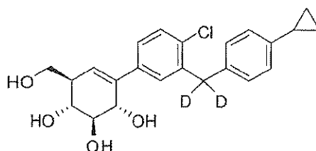
(1R,2S,3S,6R)-4-(4-chloro-3-((4-cyclopropylphenyl)methyl- d_2 )phenyl)-6-(hydroxymethyl)cyclohex-4-ene-1,2,3-triol;
