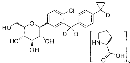
(2S,3R,4R,5S,6R)-2-(4-chloro-3-((4-(cyclopropyl-1- d )phenyl)methyl- d 2 )phenyl)-6-(hydroxymethyl)tetrahydro-2 H -pyran-3,4,5-triol, bis(L-proline) complex.
