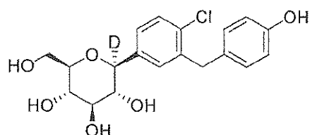
(2S,3R,4R,5S,6R)-2-(4-chloro-3-(4-hydroxybenzyl)phenyl)-6-(hydroxymethyl)tetrahydro-2H-pyran-2- d_3 ,4,5-triol;
