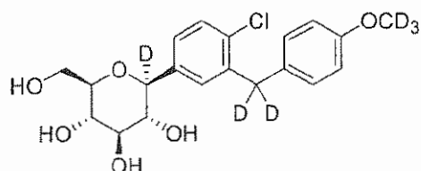
(2S,3R,4R,5S,6R)-2-(4-chloro-3-((4-(methoxy- d_3 )phenyl)methyl- d_2 )phenyl)-6-(hydroxymethyl)tetrahydro-2H-pyran-2- d -3,4,5-triol;
