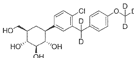
15 (1R,2R,3S,4S,6R)-4-(4-chloro-3-((4-(methoxy- d_3 )phenyl)methyl- d_2 )phenyl)-6-(hydroxymethyl)cyclohexane-1,2,3-triol;
