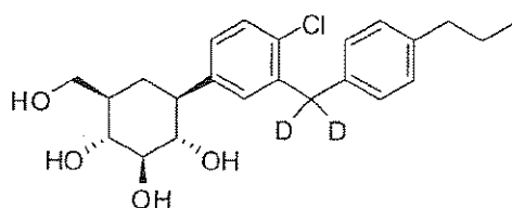
(1R,2R,3S,4S,6R)-4-(4-chloro-3-((4-propylphenyl)methyl- d_2 )phenyl)-6-(hydroxymethyl)cyclohexane-1,2,3-triol;
