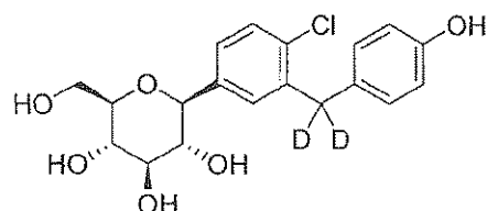
20 (2S,3R,4R,5S,6R)-2-(4-chloro-3-((4-hydroxyphenyl)methyl- d_2 )phenyl)-6-(hydroxymethyl)tetrahydro-2H-pyran-3,4,5-triol;
