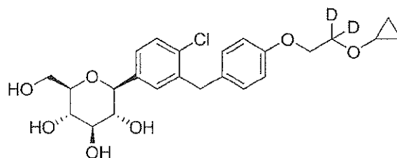
(2S,3R,4R,5S,6R)-2-(4-chloro-3-(4-(2-cyclopropoxy(ethoxy-2,2- d_2 ))benzyl)phenyl)-6-(hydroxymethyl)-tetrahydro-2H-pyran-3,4,5-triol;
