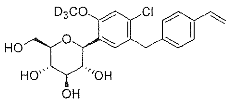
(2S,3R,4R,5S,6R)-2-(4-chloro-5-(4-vinylbenzyl)-2-(methoxy- d 3 )phenyl)-6-(hydroxymethyl)tetrahydro-2 H -pyran-3,4,5-triol;
