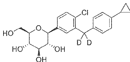
(2S,3R,4R,5S,6R)-2-(4-chloro-3-((4-cyclopropylphenyl)methyl- d_2 )phenyl)-6-(hydroxymethyl)tetrahydro-2H-pyran-3,4,5-triol; and
