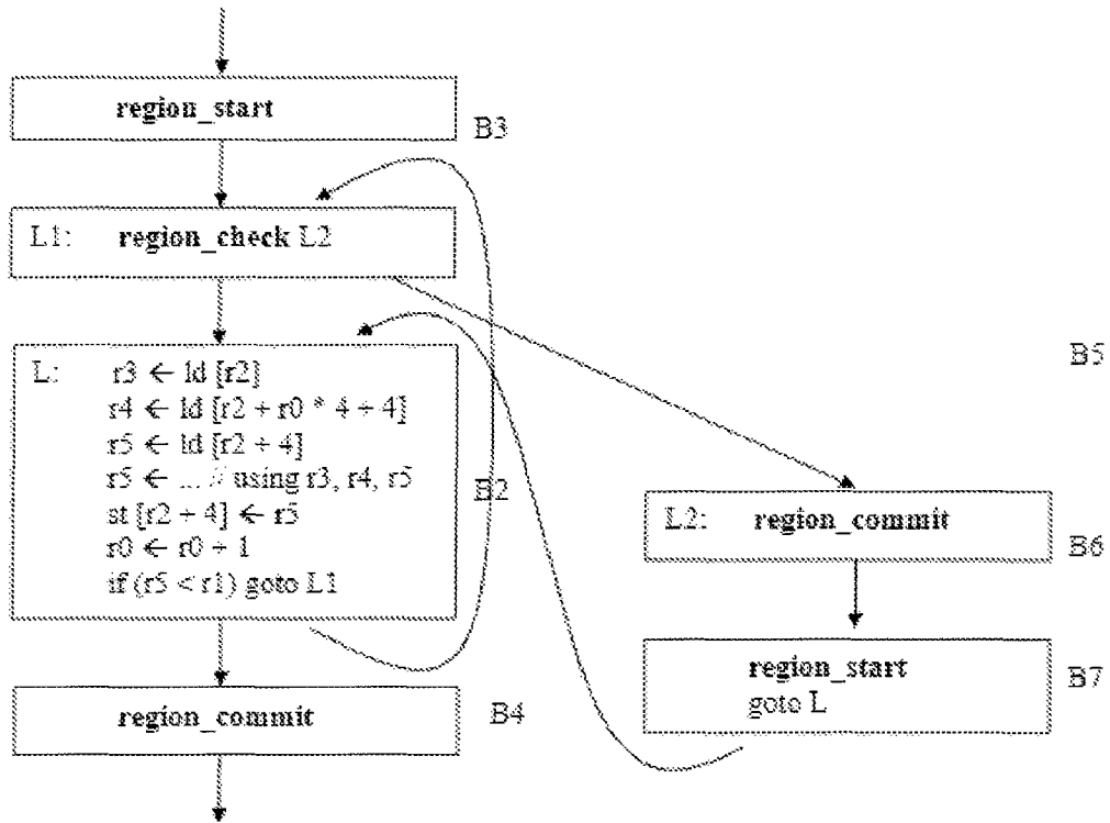
Pseudo Code D: Code region with conditional commit code inserted
