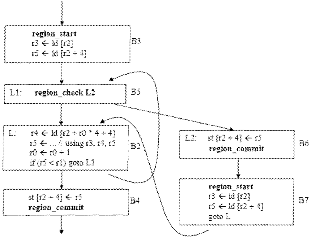
Pseudo Code E: Code region after optimization
