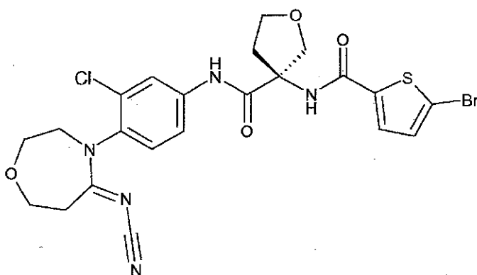
(S)-5-bromo-thiophene-2-carboxylic acid- N -{3-[3-chloro-4-(5-cyanimin-[1.4]oxazepan-4-yl)-phenylcarbamoyl]-tetrahydrofuran-3-yl}-amide
