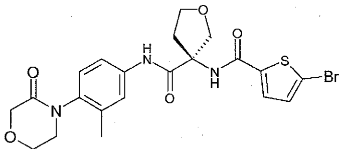
(S)-5-ethynyl-thiophene-2-carboxylic acid- N -{3-[4-(3-oxo-morpholin-4-yl)-phenylcarbamoyl]-tetrahydro-thiophen-3-yl}-amide
