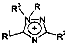
(IVg')
