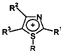
(IVo')
