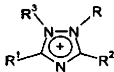
(IVg)
