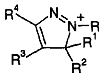
(IVg')
