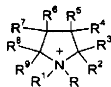
(IVs)
