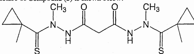
Compound (1)
