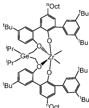
Catalyst 4 Single-Chain Catalyst
