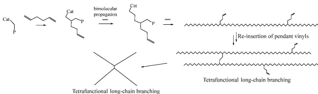
Scheme 2: Long-Chain Branching via Diene Incorporation
