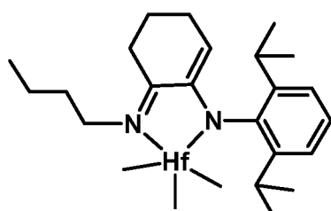
Catalyst 1: Dual-chain catalyst
