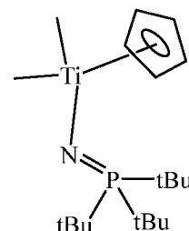
Catalyst 3 Single-chain catalyst
