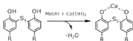
(Scheme II)
