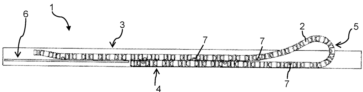
FIG. 6 (PRIOR ART)
