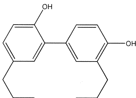
tetrahydrohonokiol
