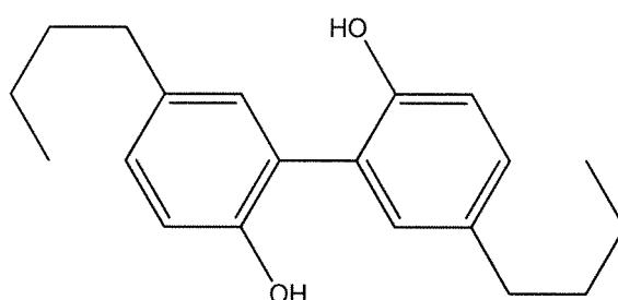
5,5'-di-n-butyl-biphenyl-2,2'-diol
