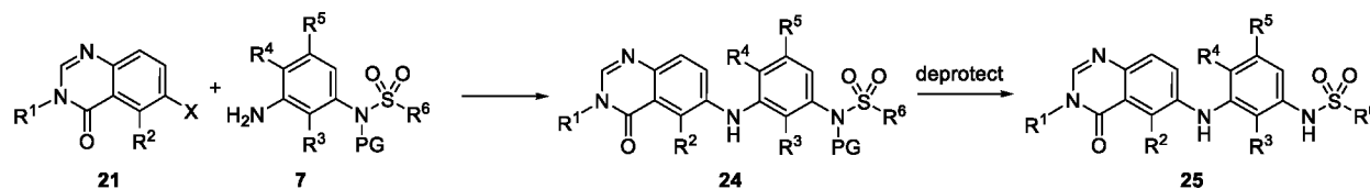
Scheme 9
