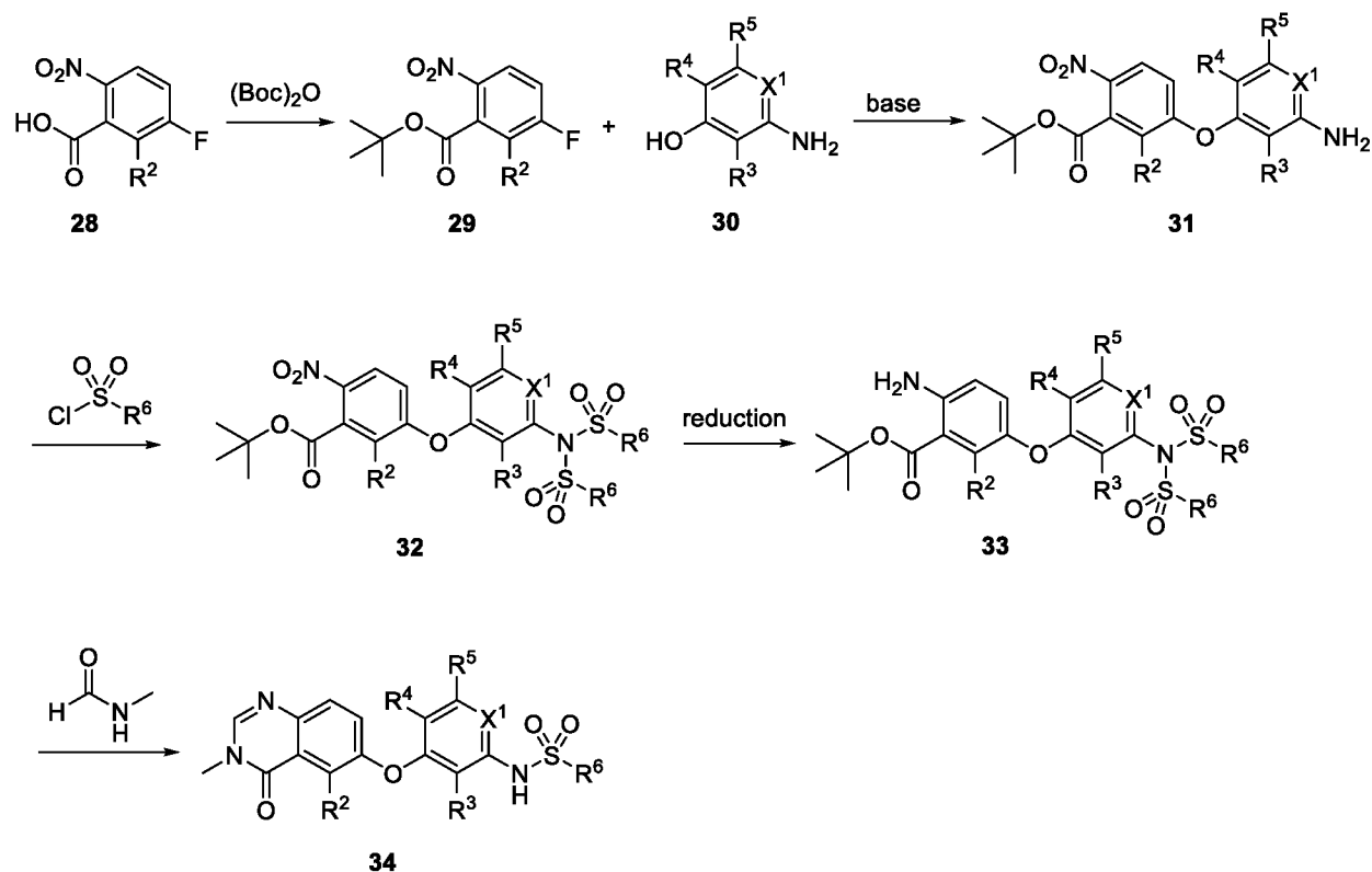
Scheme 11
