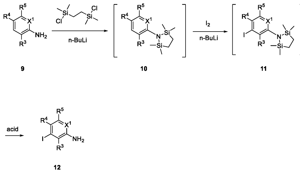
Scheme 3
