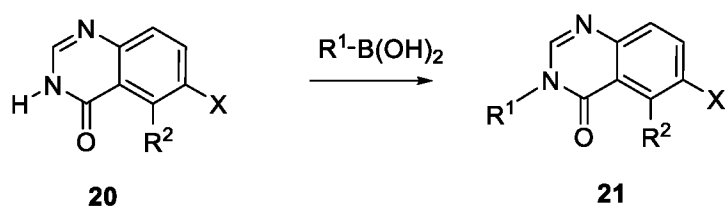
Scheme 7
