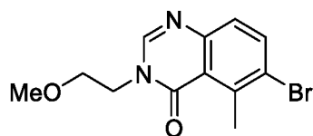
6-bromo-3-(2-methoxyethyl)-5-methylquinazolin-4(3H)-one
