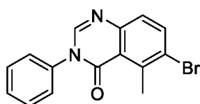
6-bromo-5-methyl-3-phenylquinazolin-4(3H)-one
