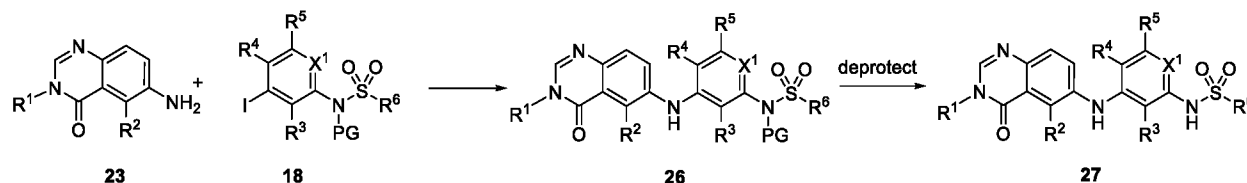
Scheme 10
