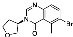
(R)-6-bromo-5-methyl-3-(tetrahydrofuran-3-yl)quinazolin-4(3H)-one
