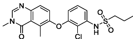
N-(2-chloro-3-((3,5-dimethyl-4-oxo-3,4-dihydroquinazolin-6-yl)oxy)phenyl)propane-1-sulfonamide
