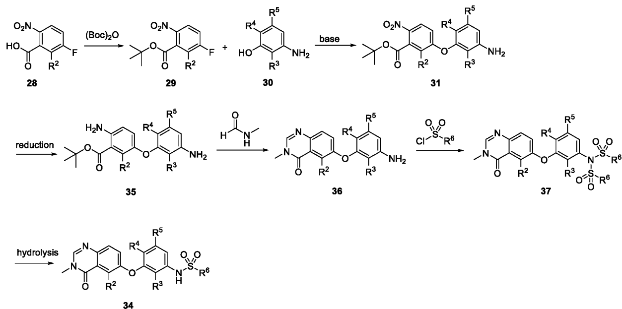
Scheme 12
