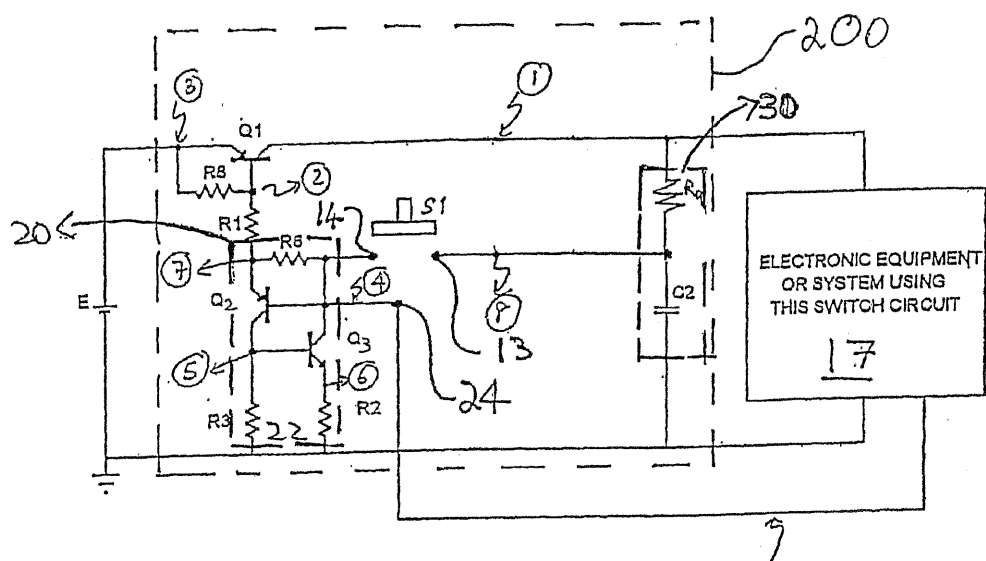
FIGURE 5 : AUTOMATIC POWER-DOWN WITH ELECTRICAL CONNECTION AT POINT (4)
