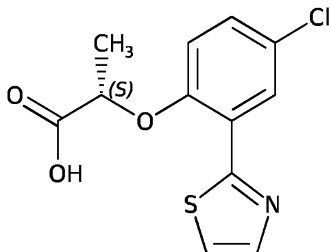
Compound A-13
