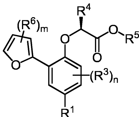
Formula (XIV)
