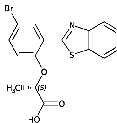
Compound A-12
