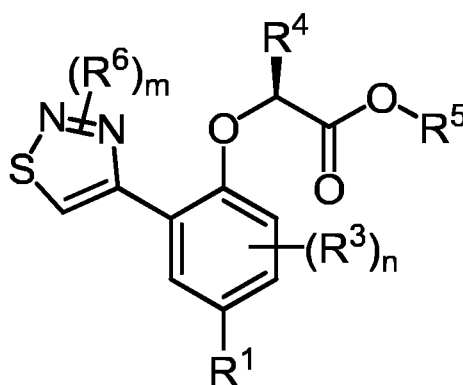
Formula (XVII)
