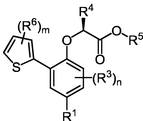
Formula (XIII)
