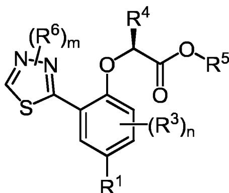
Formula (XVIII)
