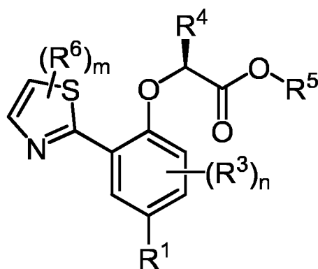
Formula (VII)
