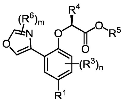
Formula (XVI)
