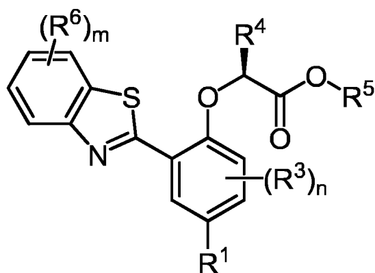
Formula (X)
