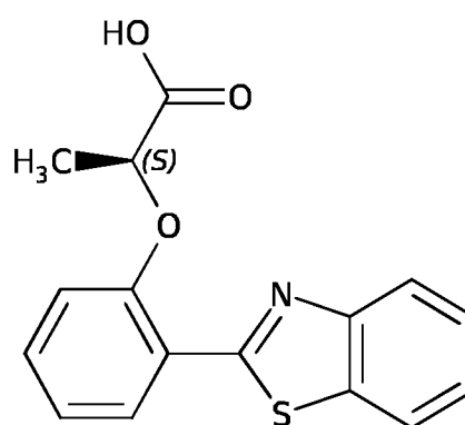
Compound A-28
