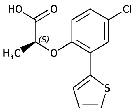
Compound A-25
