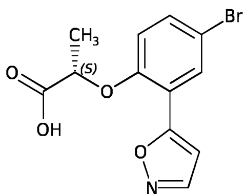
Compound A-22
