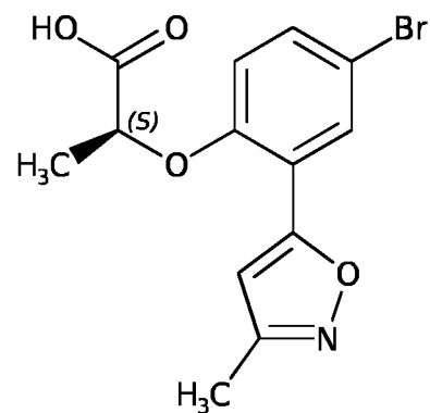
Compound A-16
