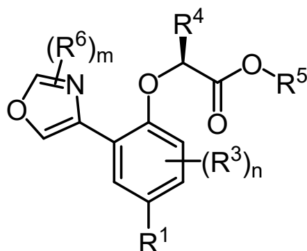
Formula (XVI)
