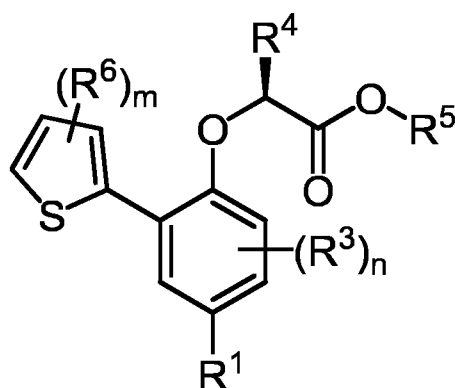
Formula (XIII)
