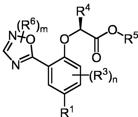
Formula (IX)
