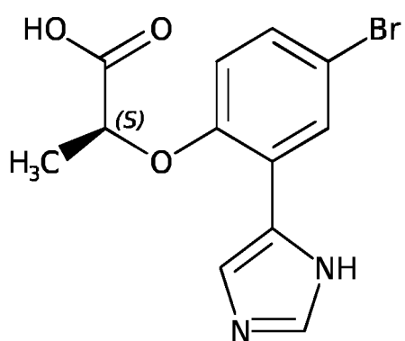
Compound A-19
