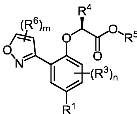
Formula (III)
