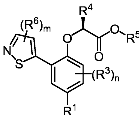
Formula (V)
