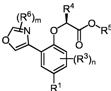
Formula (XVI)
