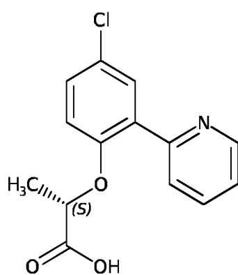
Compound A-7
