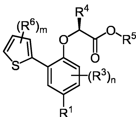
Formula (XIII)
