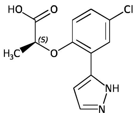
Compound A-24
