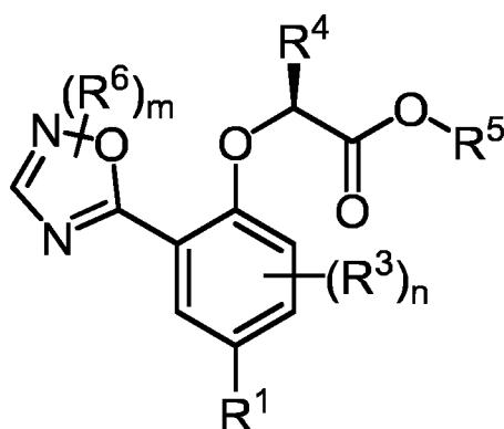
Formula (IX)
