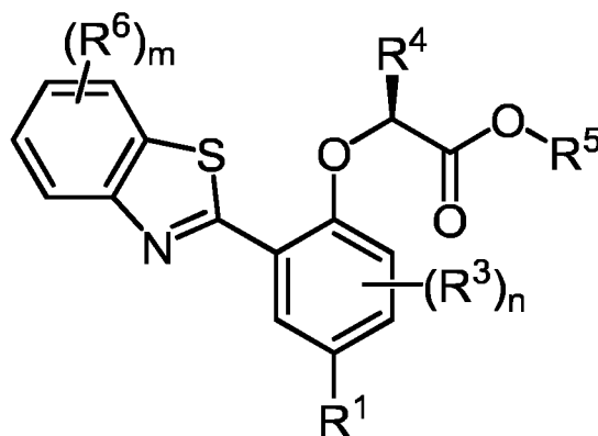
Formula (X)
