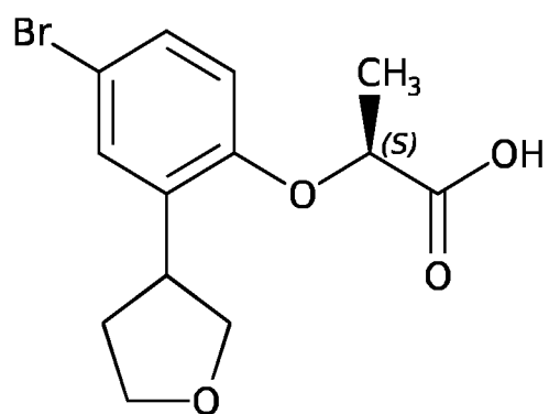
Compound A-20
