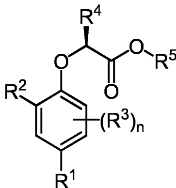
Formula (I)
