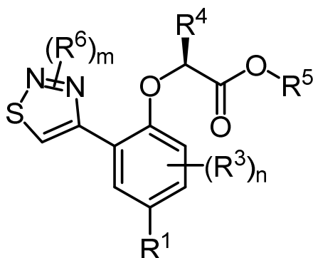
Formula (XVII)
