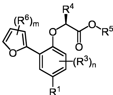
Formula (XIV)
