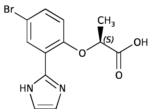
Compound A-18
