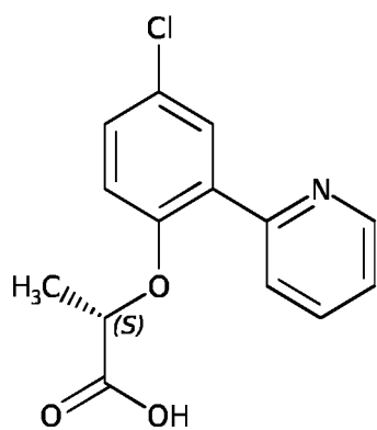
Compound A-7
