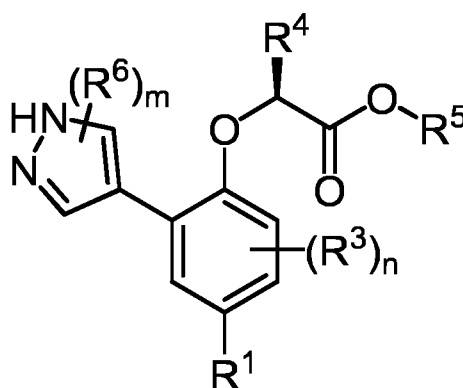
Formula (XII)
