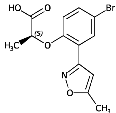
Compound A-8
