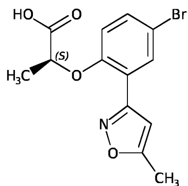
Compound A-8
