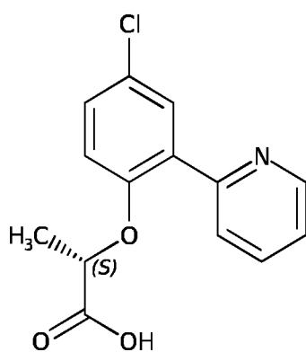
Compound A-7
