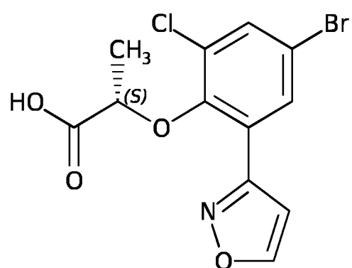
Compound A-6
