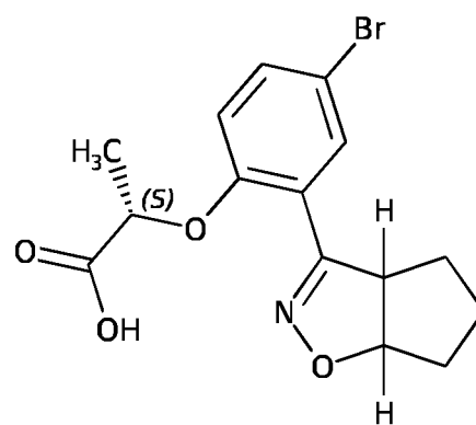
Compound A-10
