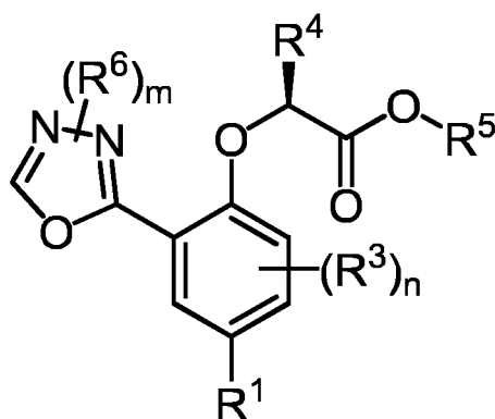
Formula (XV)
