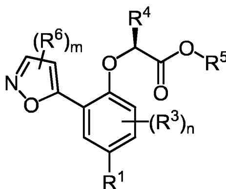
Formula (II)
