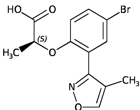
Compound A-5
