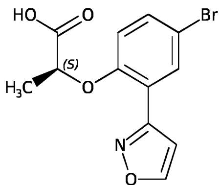
Compound A-17
