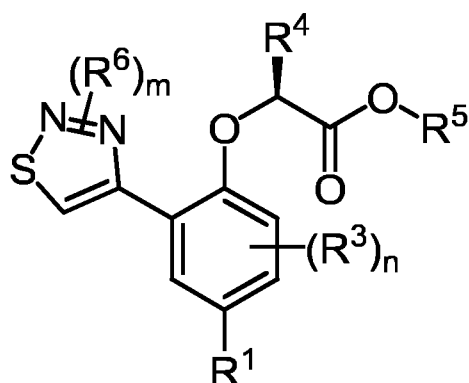
Formula (XVII)
