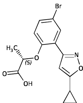
Compound A-11
