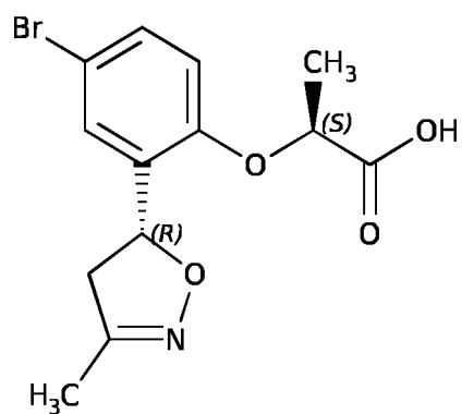
Compound A-15
