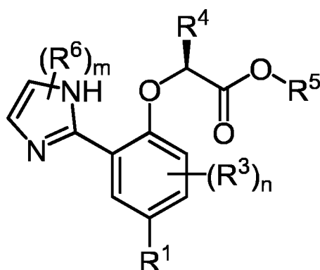
Formula (VIII)
