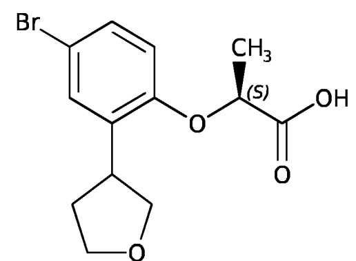
Compound A-20
