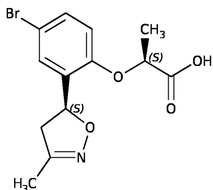
Compound A-14
