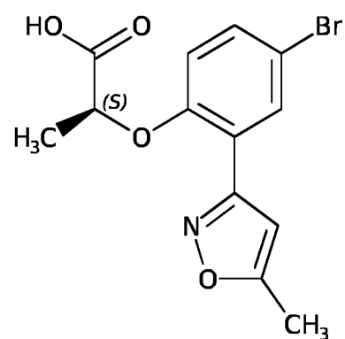
Compound A-8
