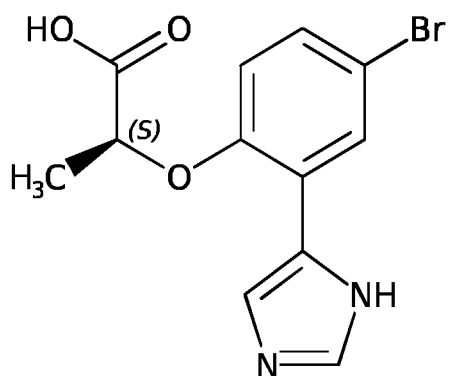
Compound A-19
