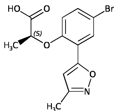
Compound A-16
