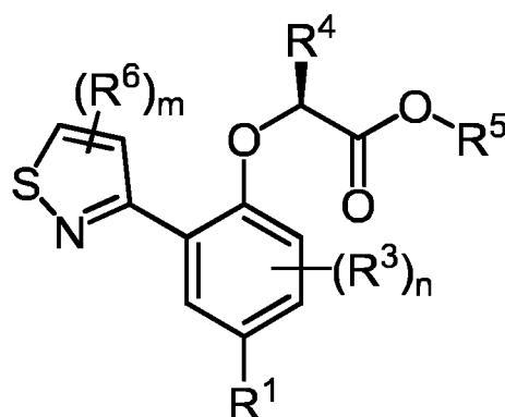
Formula (VI)
