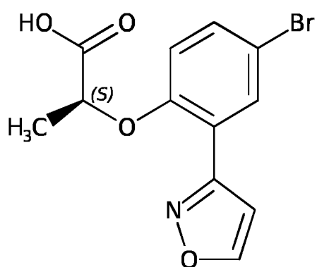
Compound A-17
