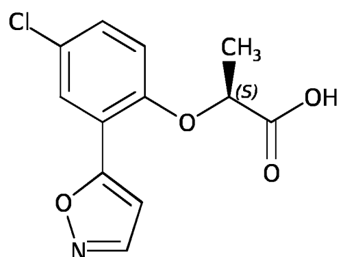
Compound A-26
