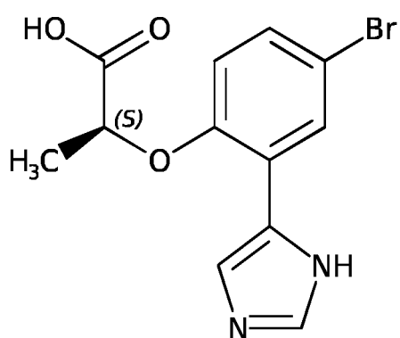
Compound A-19
