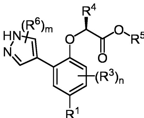
Formula (XII)
