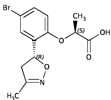
Compound A-15
