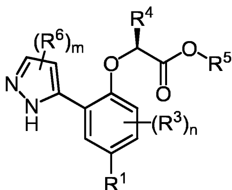
Formula (XI)
