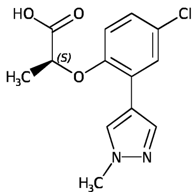
Compound A-27
