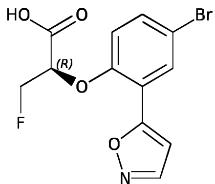
Compound A-21
