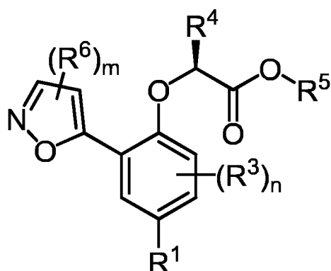
Formula (II)
