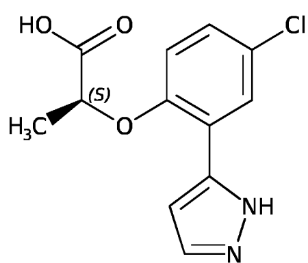
Compound A-24
