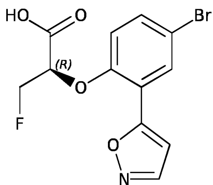
Compound A-21
