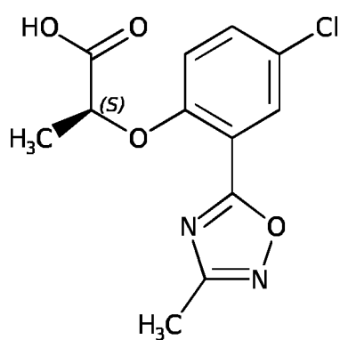
Compound A-9
