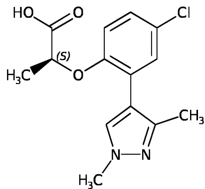
Compound A-23
