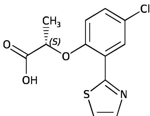
Compound A-13
