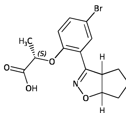
Compound A-10
