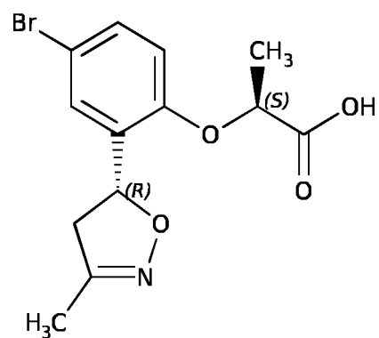
Compound A-15
