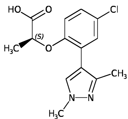
Compound A-23
