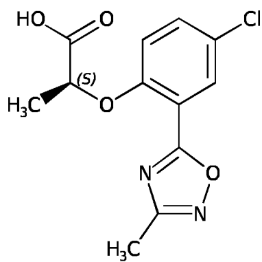
Compound A-9
