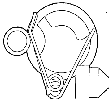
Fig. 1 (Prior art)
