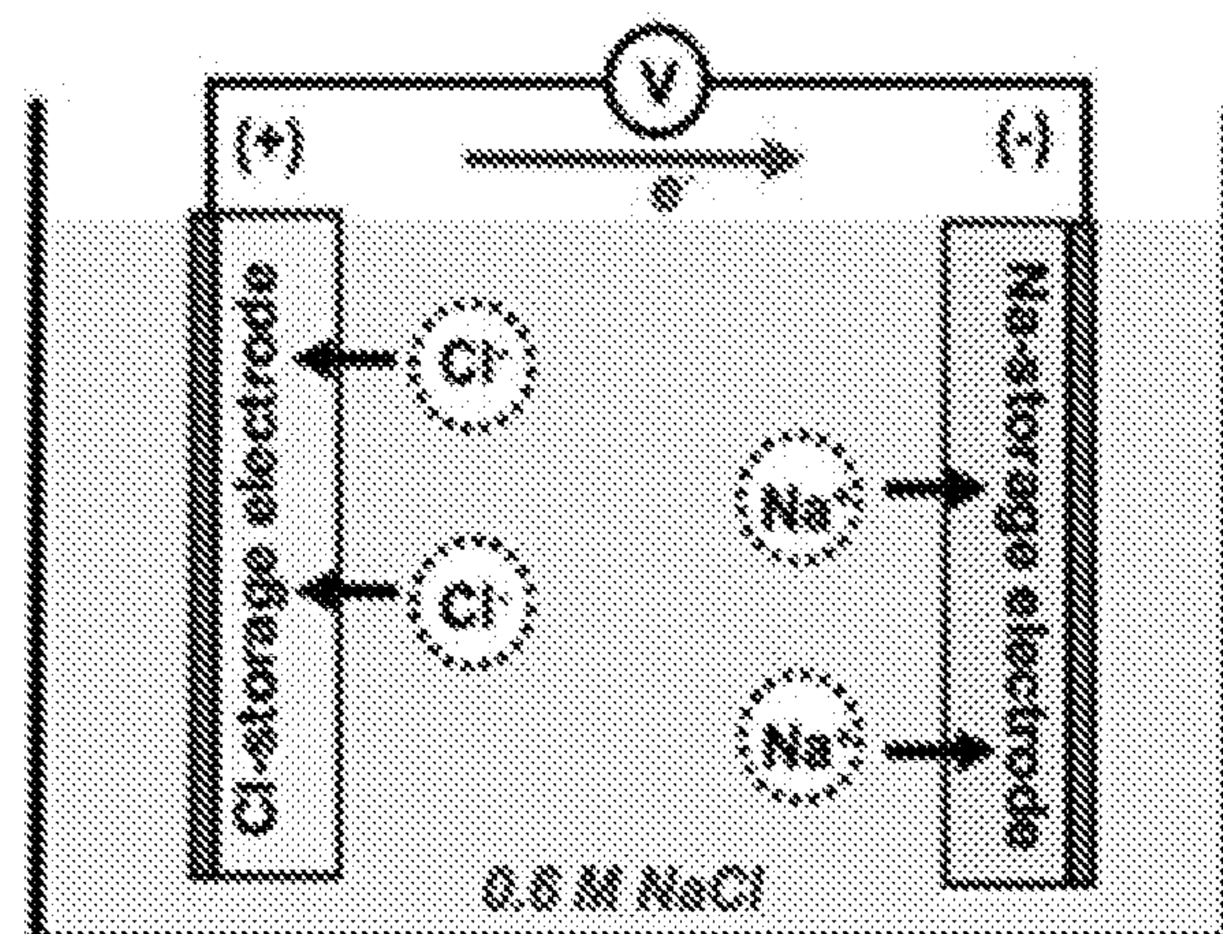
FIG. 7B Desalination (Charging)
