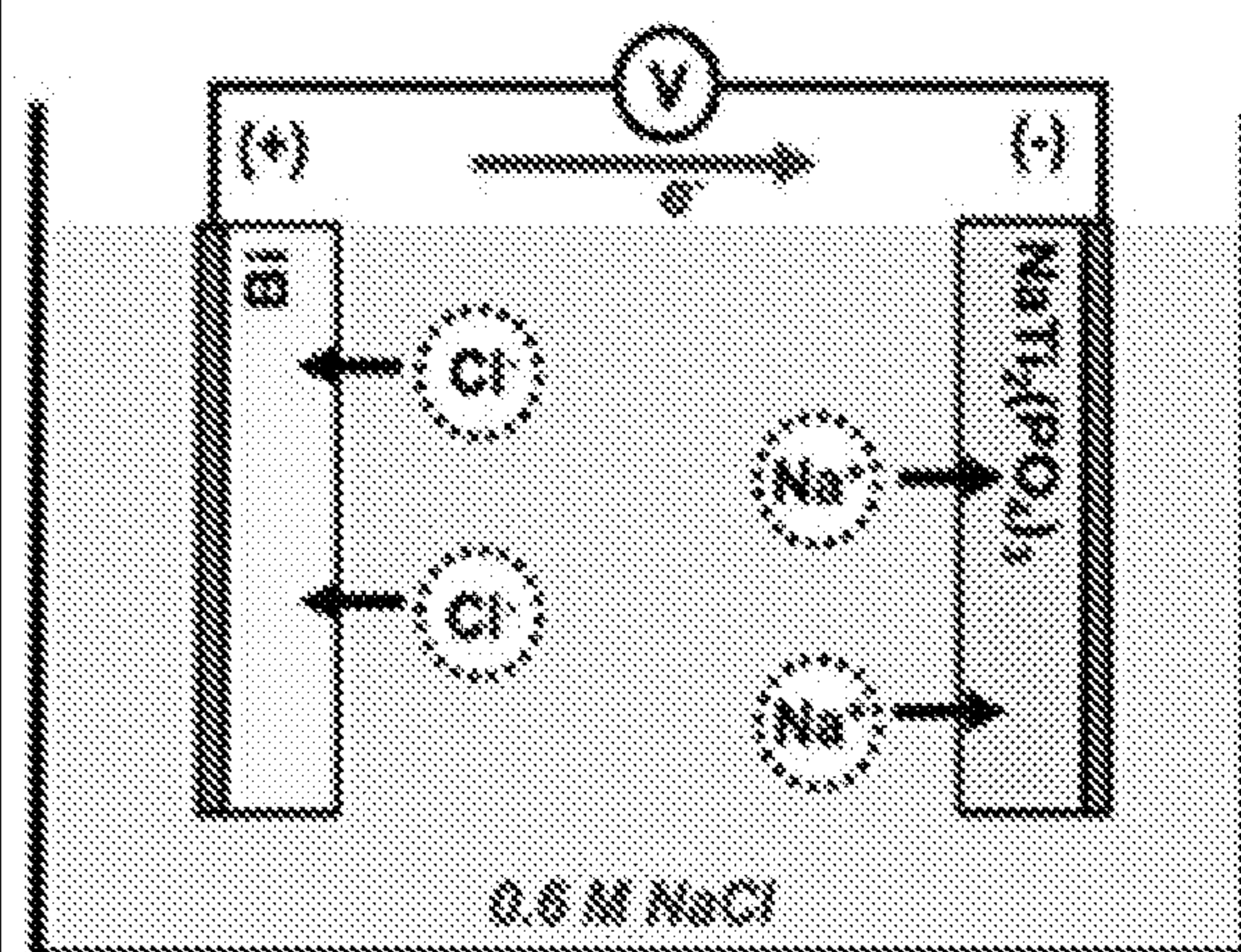
FIG. 7C Desalination (Charging)
