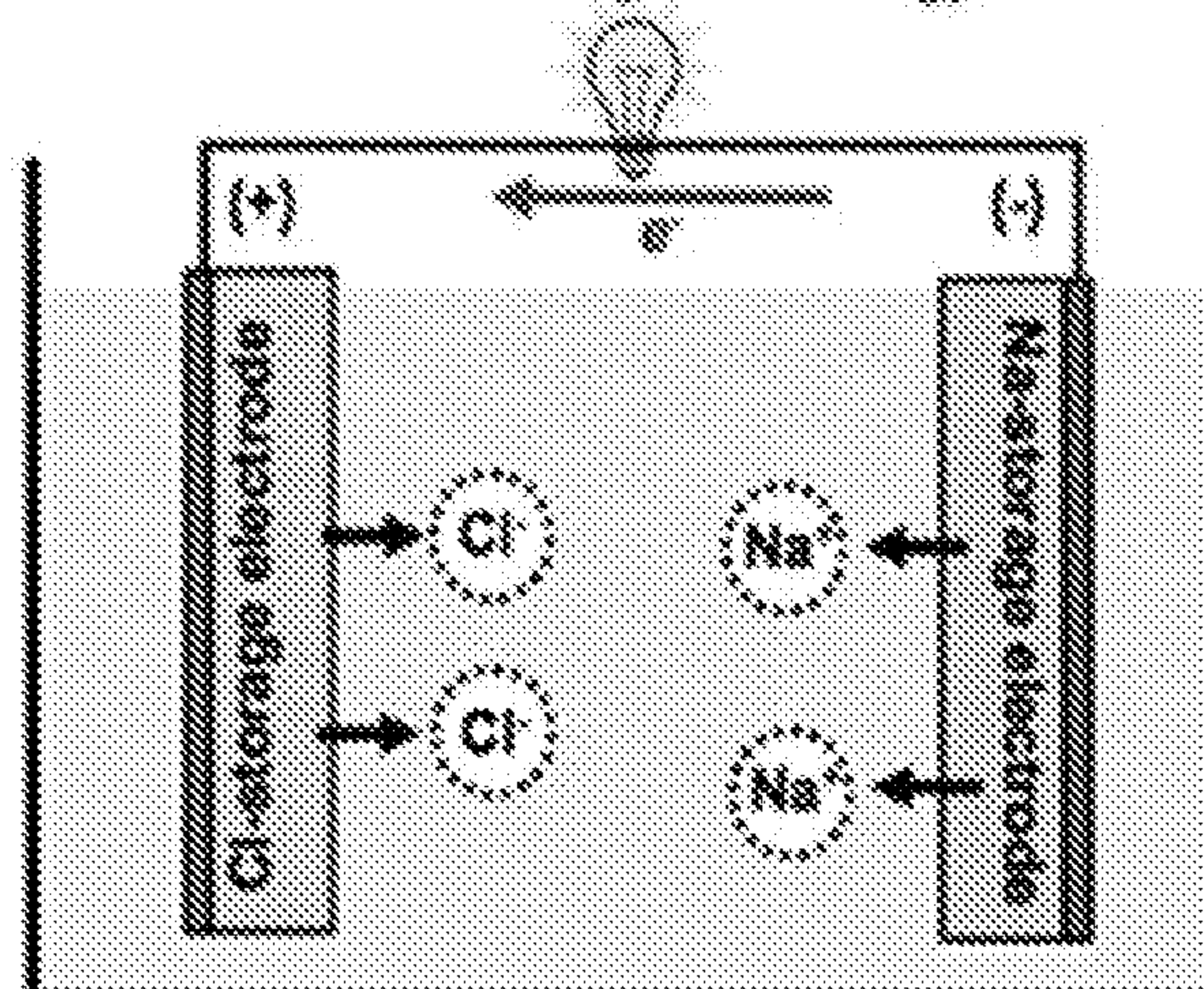
Salination (Discharging)
