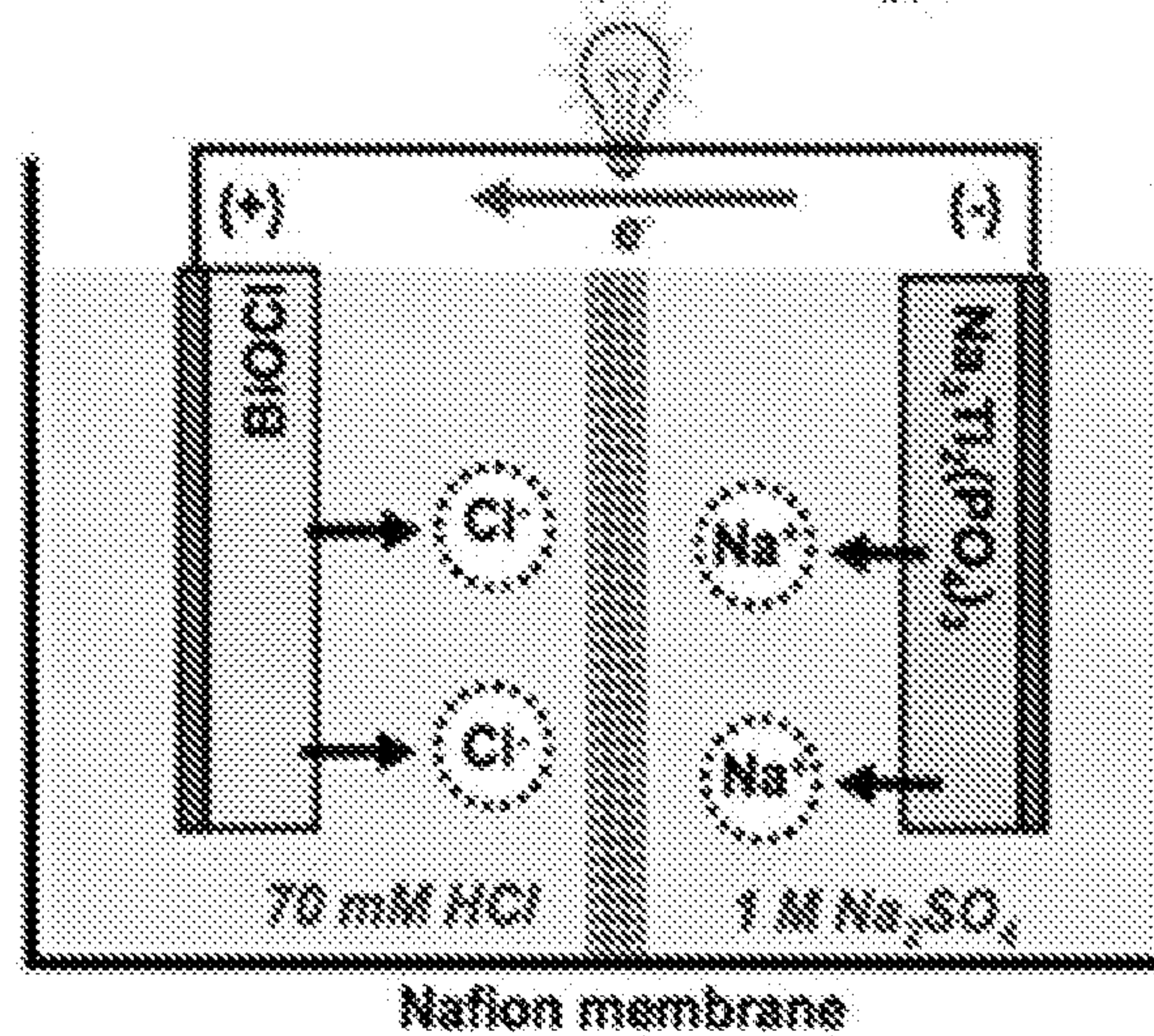
Salination (Discharging)
