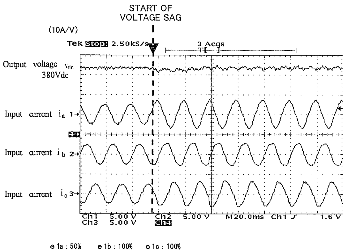
FIG. 11B VOLTAGE SAG COMPENSATION IS PERFORMED
