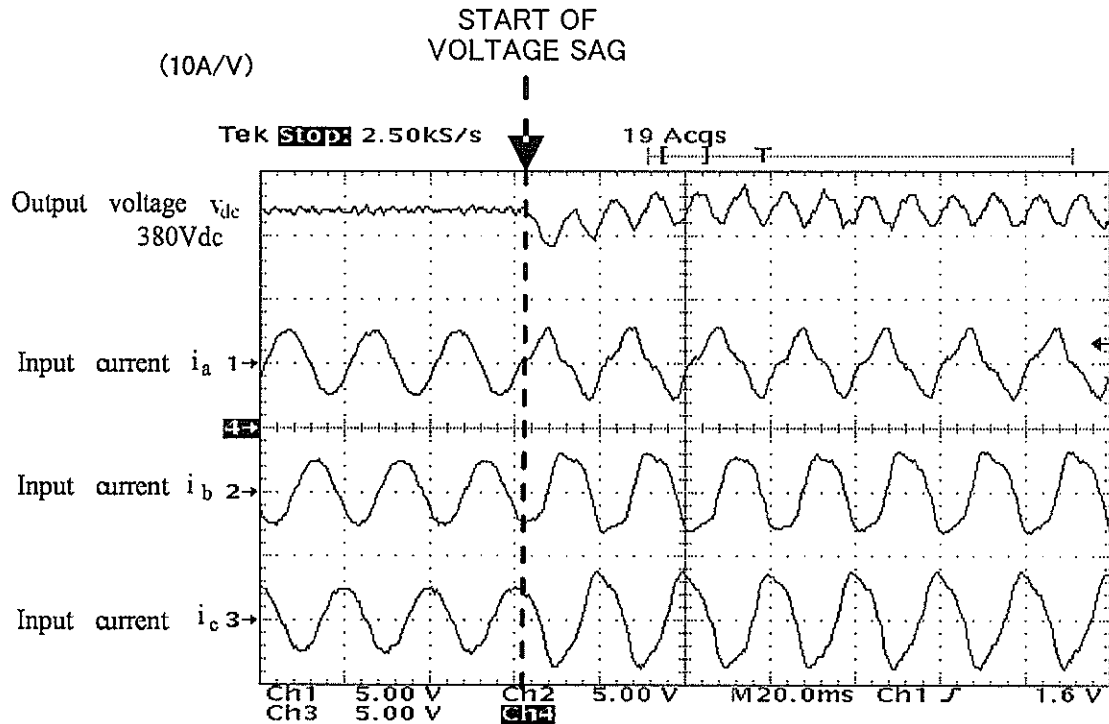
FIG. 11A COMPENSATION FOR VOLTAGE SAG IS NOT PERFORMED
