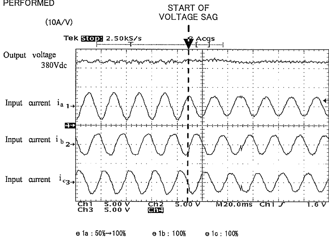
FIG. 12B VOLTAGE SAG COMPENSATION IS PERFORMED
