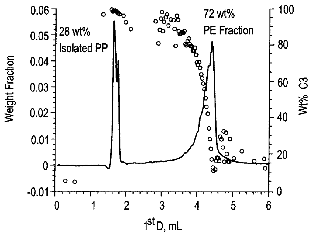
FIG. 4 HTLC of CBC1
