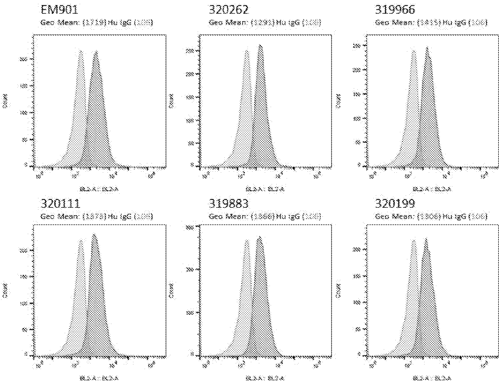
Fig 4. BCMA-Binding Antibodies Bind NCIH929 Multiple Myeloma Cells
