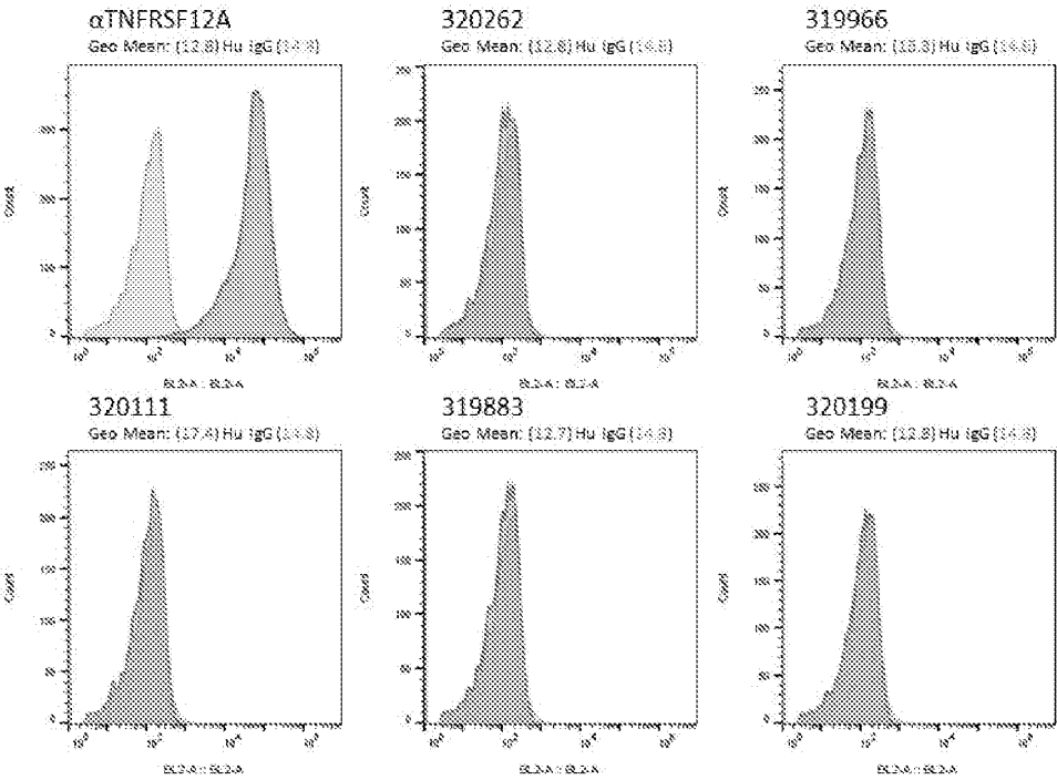
Fig 3. BCMA-Binding Antibodies Do Not Bind Hek293 Cells expressing TNFRSF12A (TWEAKR; HB6)
