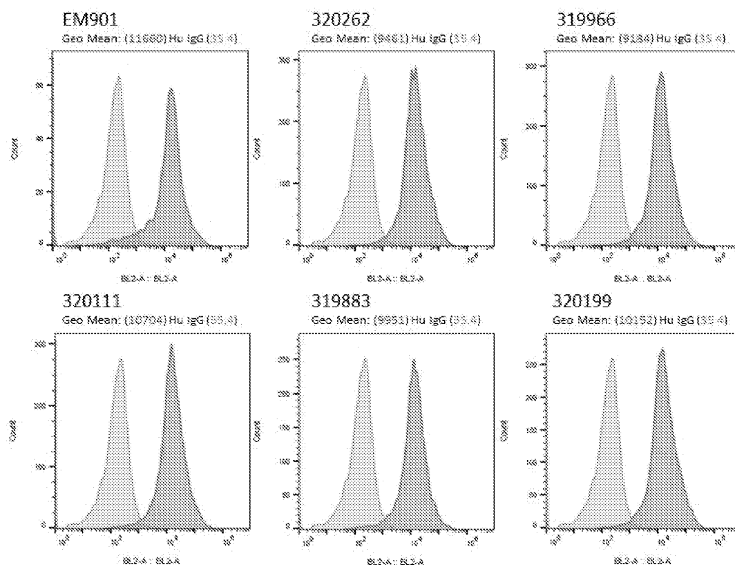
Fig 2. BCMA-Binding Antibodies Recognize C6 Cells Expressing Human BCMA
