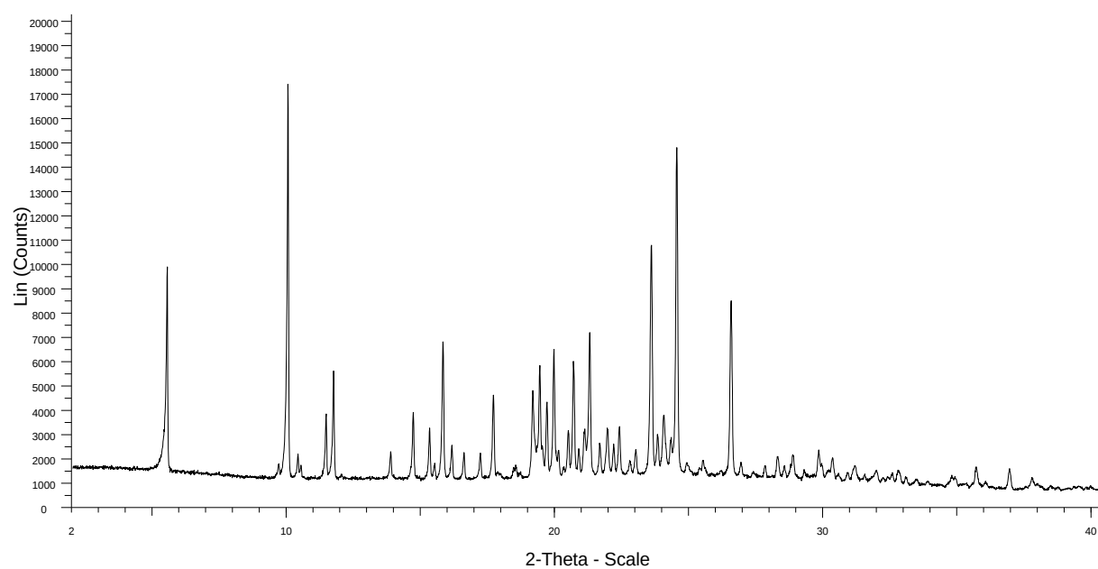
Figure 3: X-Ray powder diffractogram of the formamid solvate
