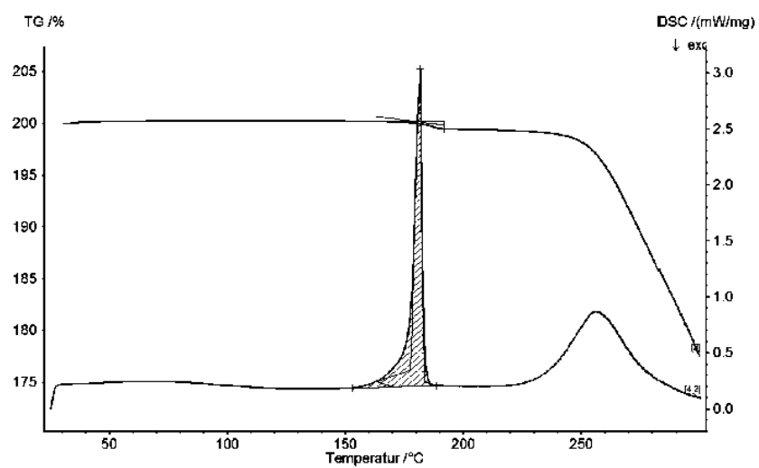
FIGURE 5: DSC- and TGA-Thermogram of anhydrate of compound (I)
