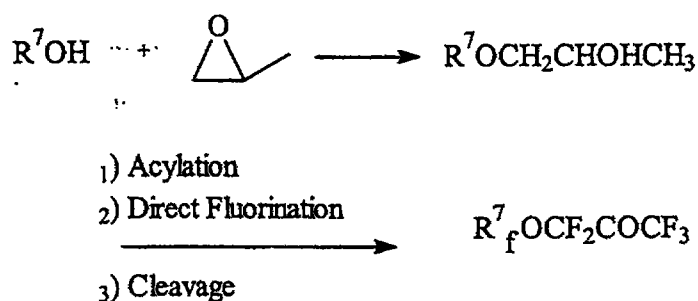
Reaction Scheme 1
