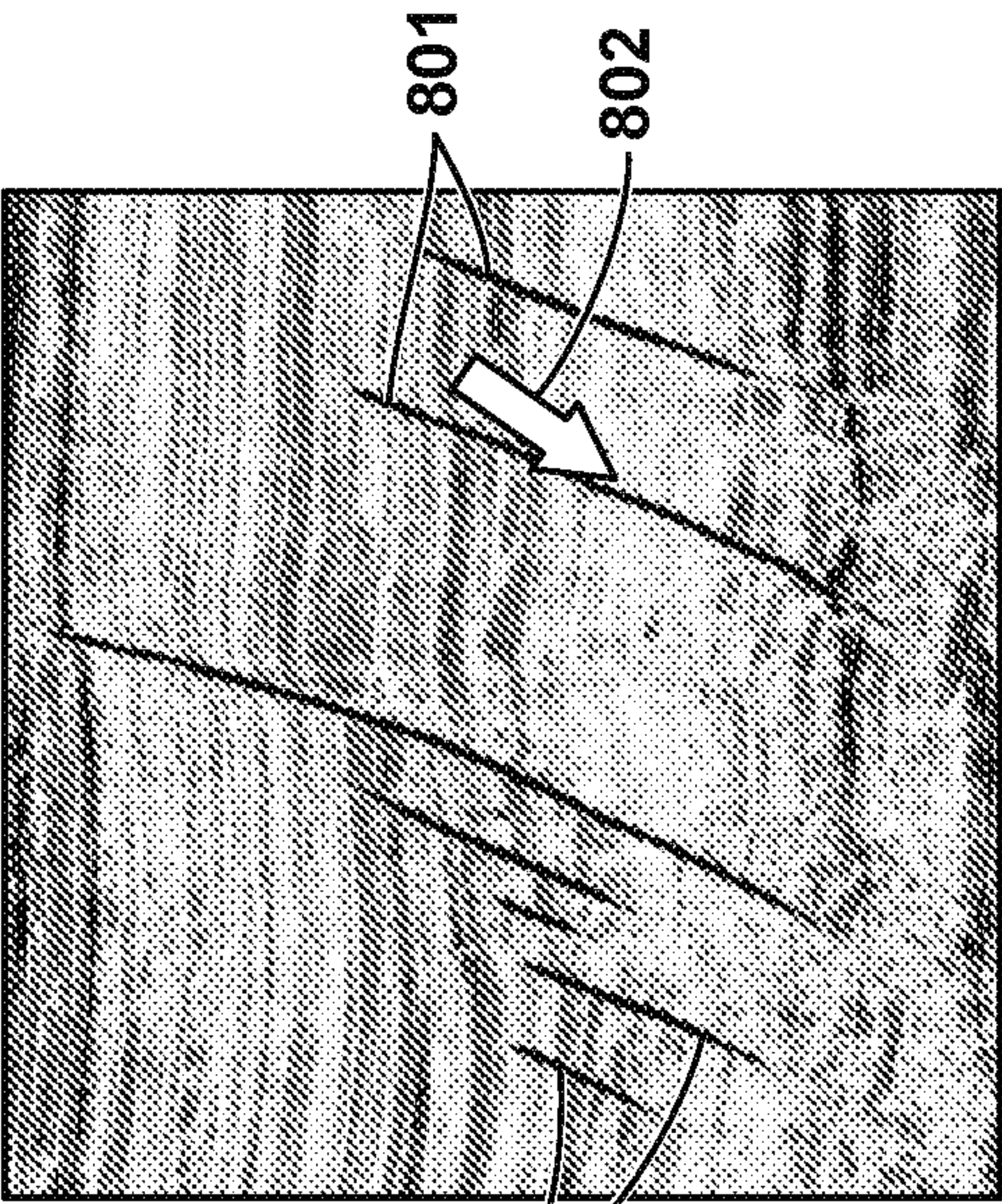
Predicted \epsilon(0,1)
