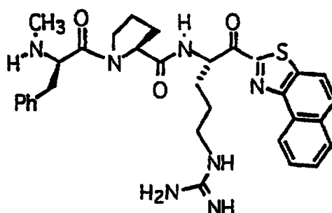
Compound 52
