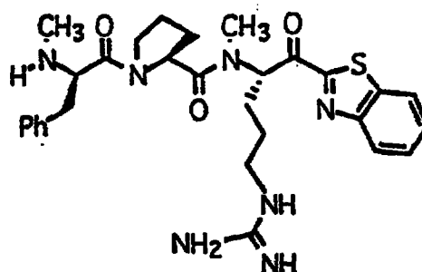
Compound 40
