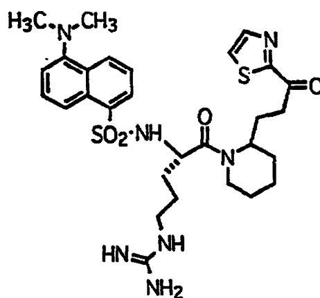
Compound 27
