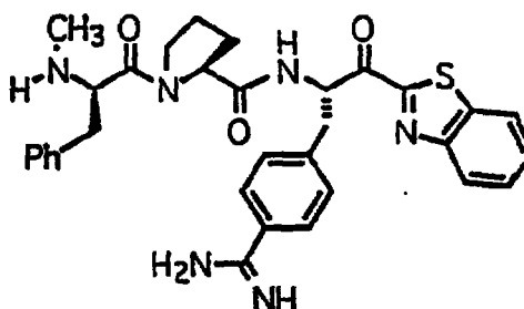
Compound 57
