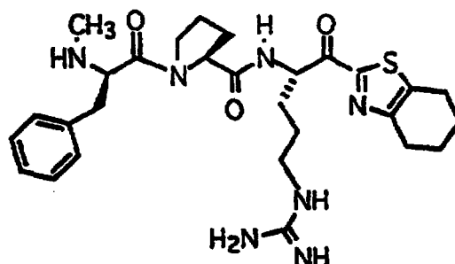
Compound 51
