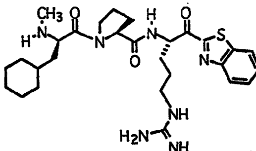
Compound 29
