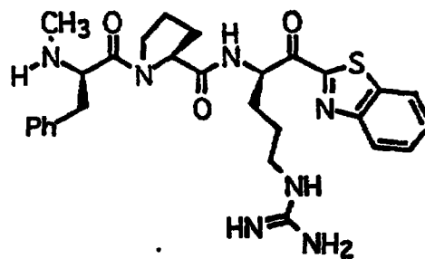
Compound 2
