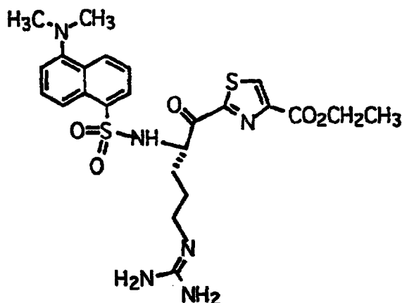
Compound 6
