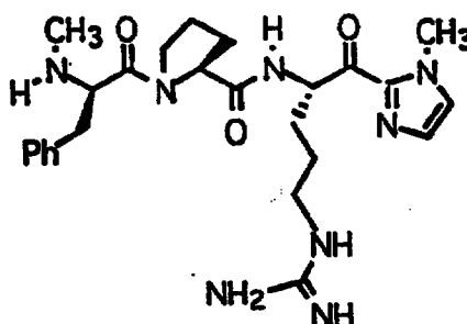
Compound 22
