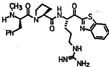
Compounds 1
