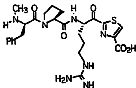
Compound 54
