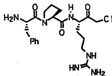
PPACK
