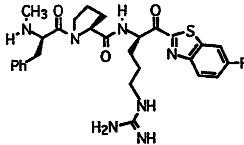
Compound 18
