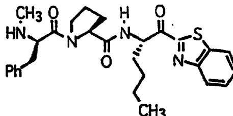
Compound 39
