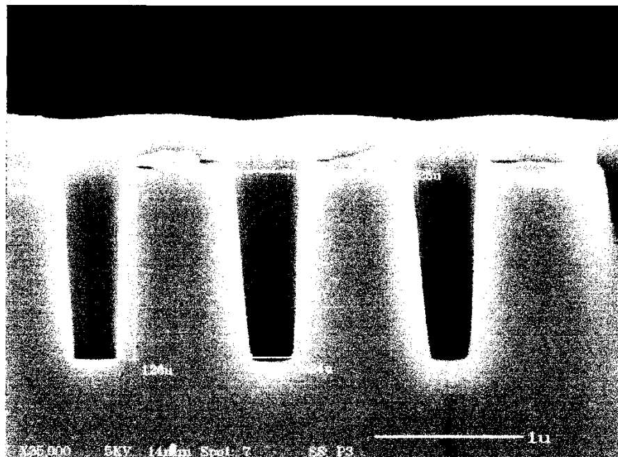
Figure 3. SEM image of C 5 F 8 O etched wafer.
