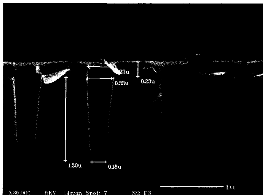
Figure 4. SEM image of C_5F_8O etched wafer
