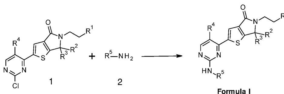
Scheme 1: Synthesis of compounds of Formula I
