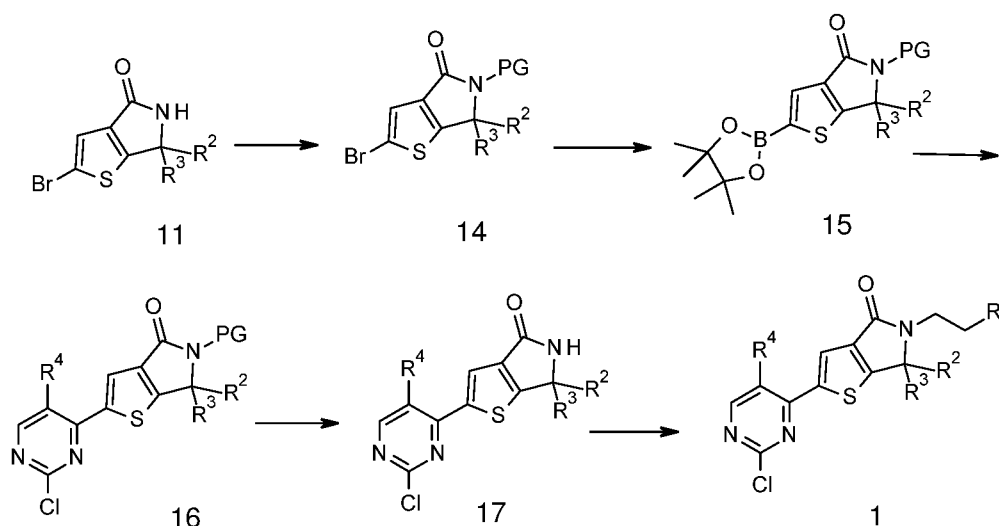
Scheme 5: Alternative synthesis of Compound 1
