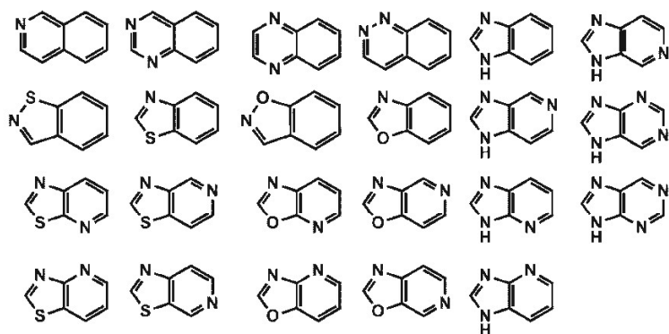
[Chemical Formula 28]
