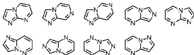
[Chemical Formula 28]
