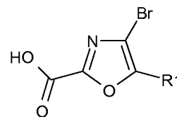
4-Bromo-oxazole-2-carboxylic acid
