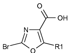
2-Bromo-oxazole-4-carboxylic acid
