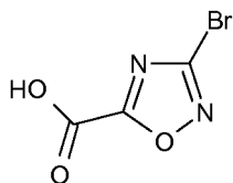
3-Bromo-[1,2,4]oxadiazole-5-carboxylic acid
