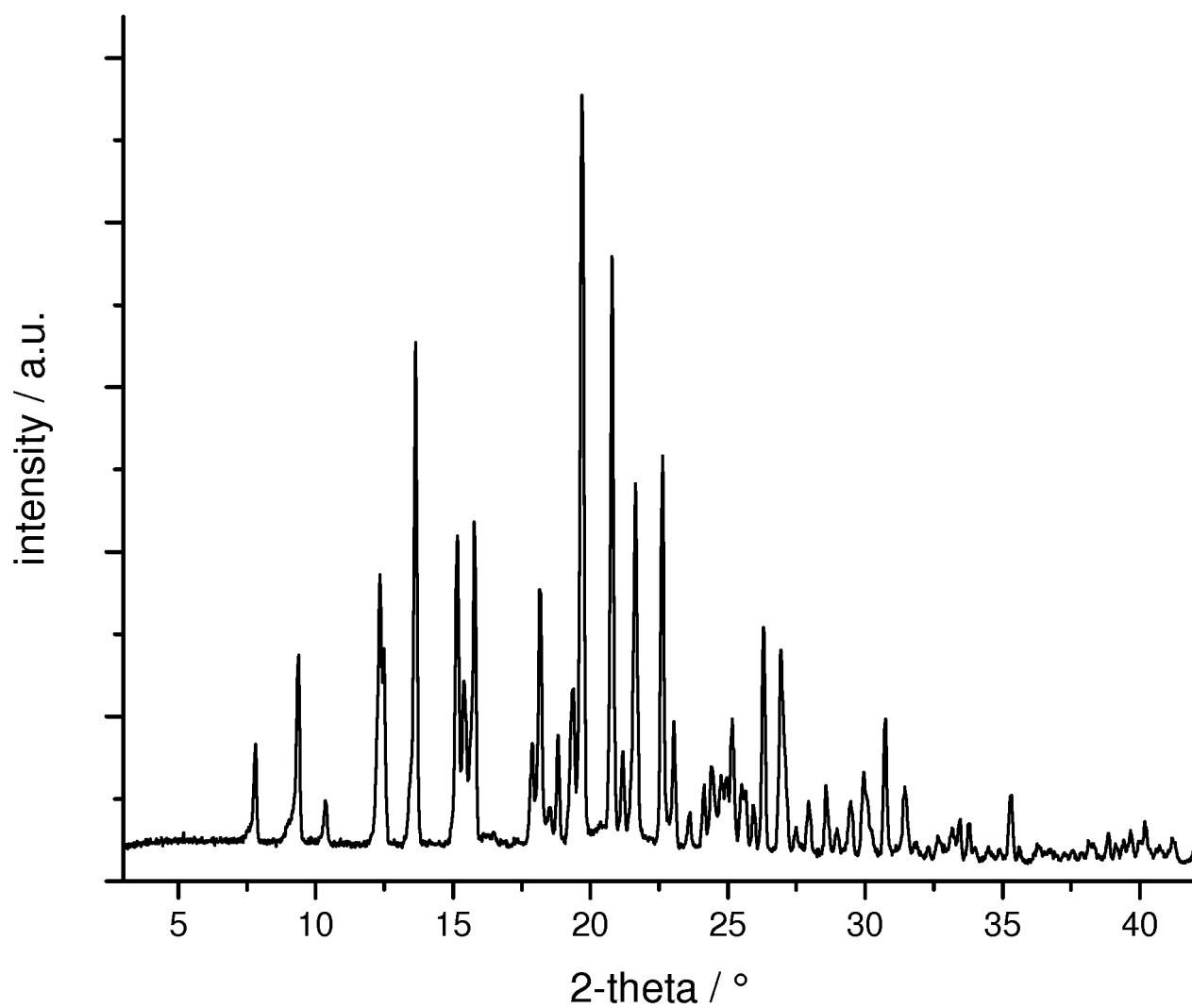
Figure 10: XRPD pattern of Form D
