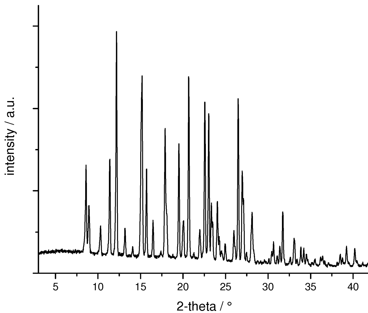
Figure 16: XRPD pattern of Form F
