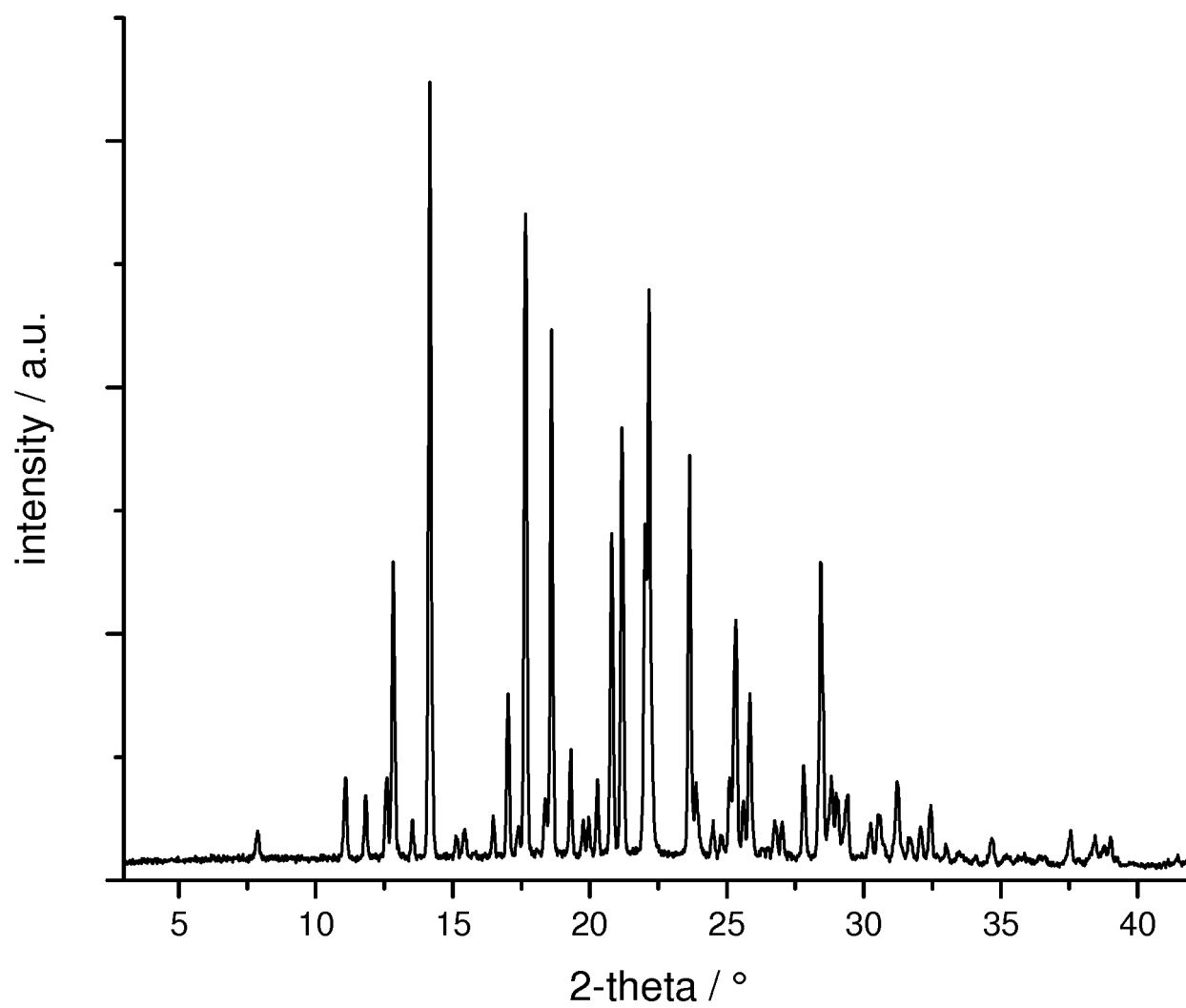
Figure 22: XRPD pattern of Form H
