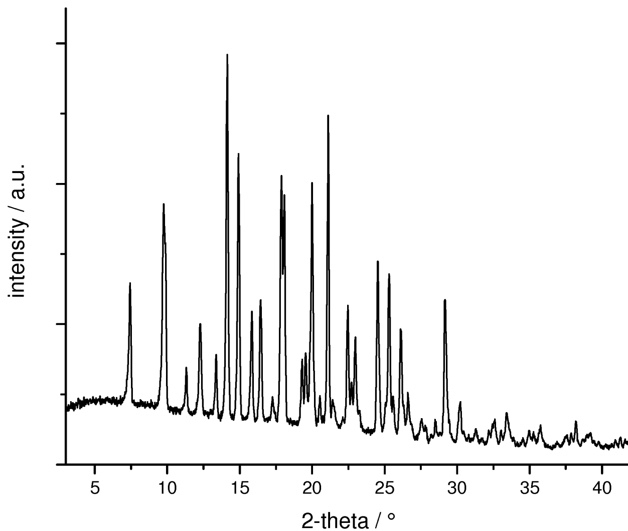
Figure 19: XRPD pattern of Form G
