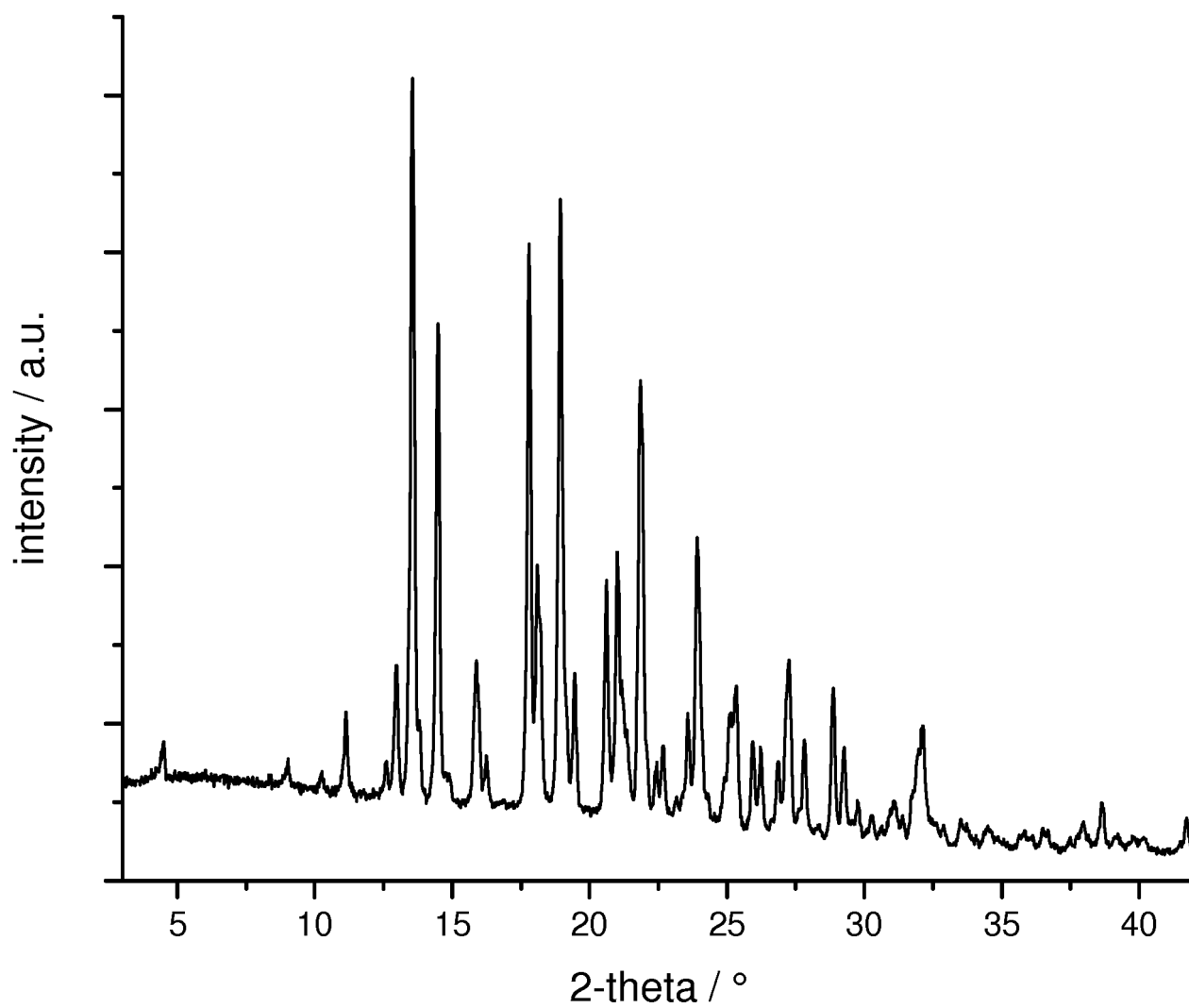
Figure 1: XRPD pattern of Form A
