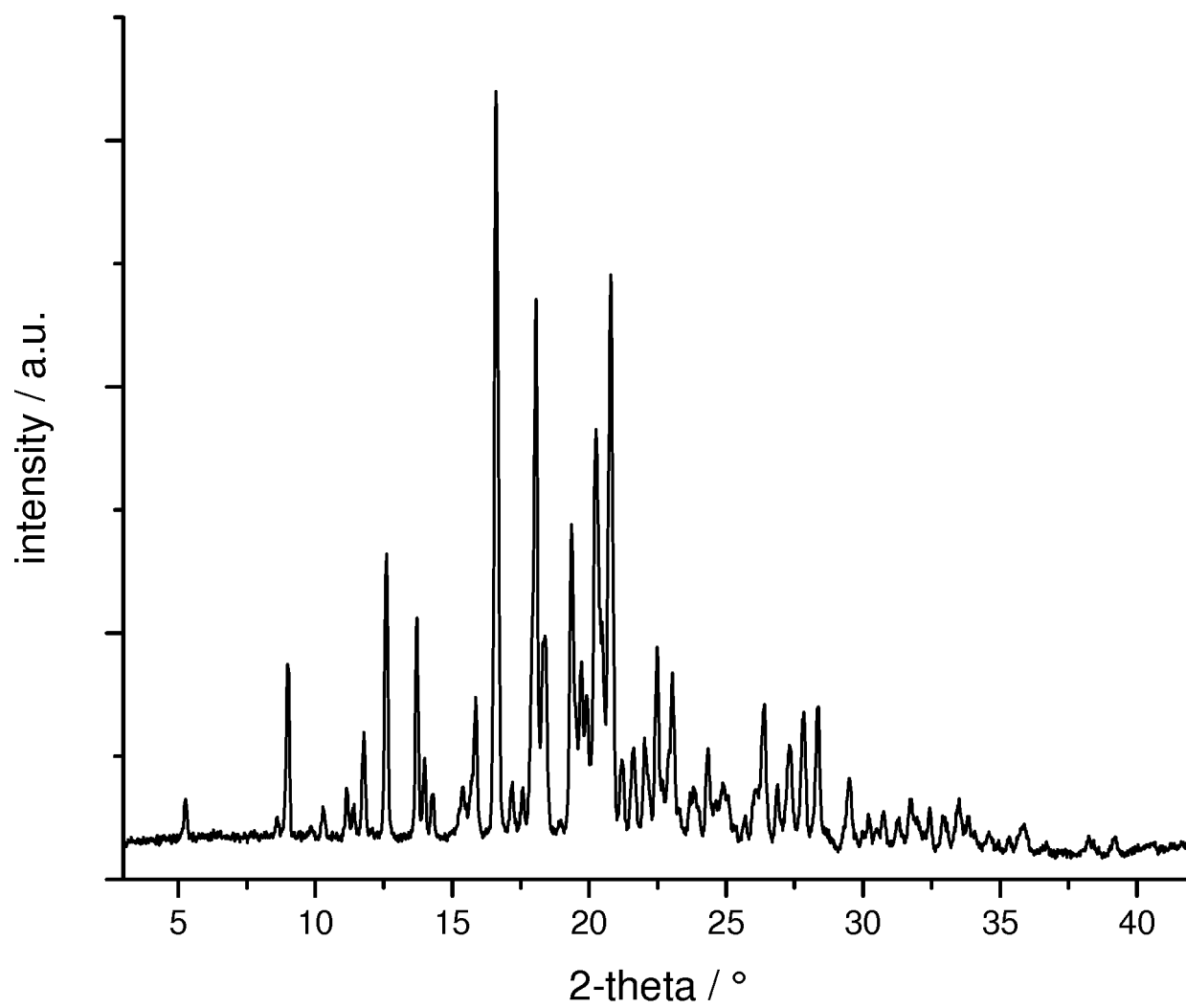
Figure 7: XRPD pattern of Form C
