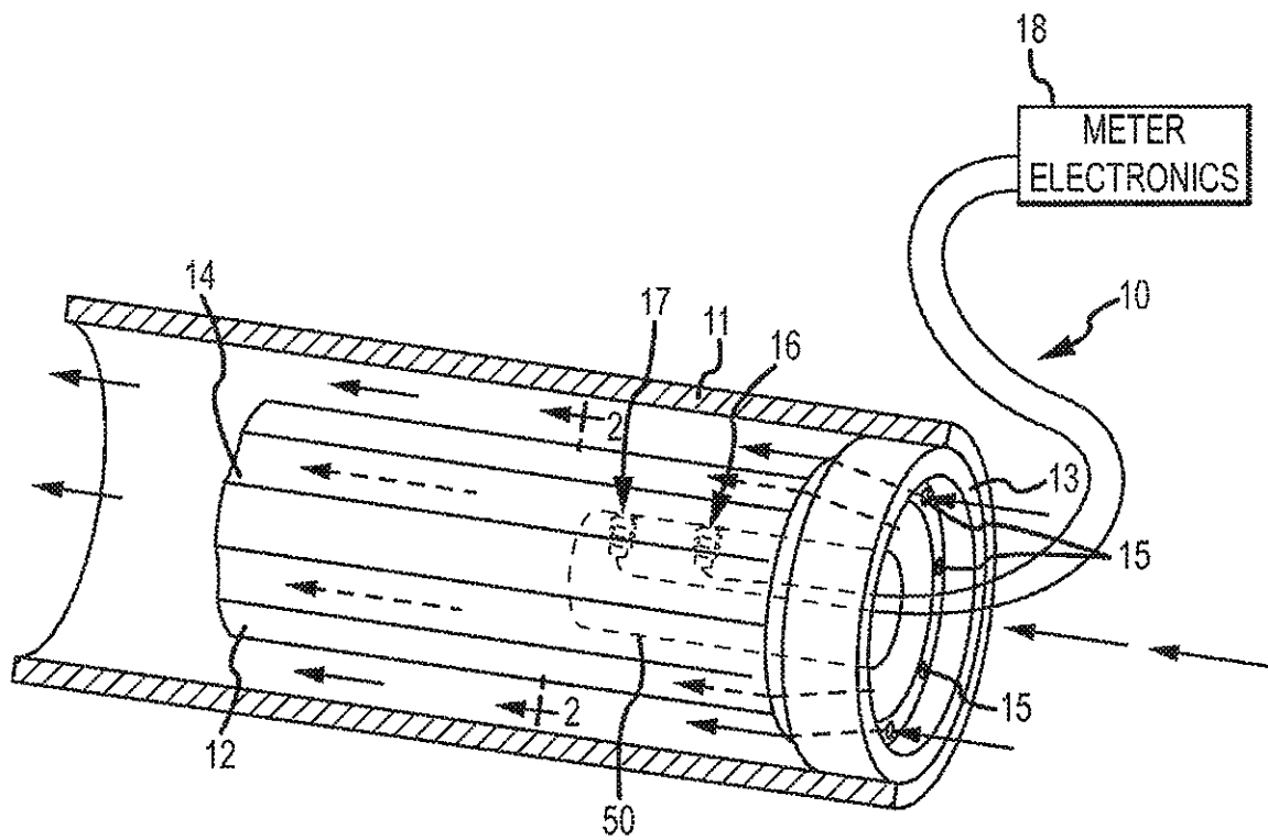
FIG. 1 (PRIOR ART)
