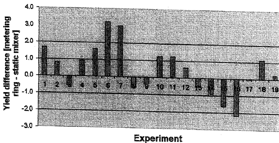
Graph A: Yield comparison with and without metering ring
