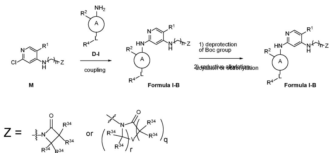
Scheme 24
