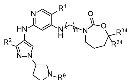
Formula IIIA.16
