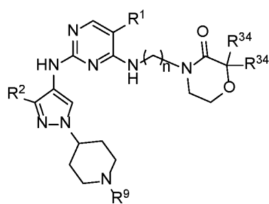
Formula IIA.4
