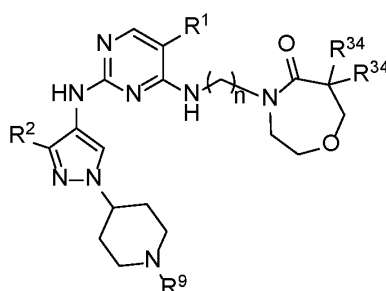
Formula IIA.1
