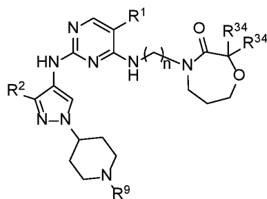
Formula IIA.3
