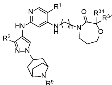
Formula IIIA.21
