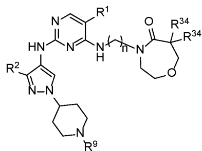
Formula IIA.1
