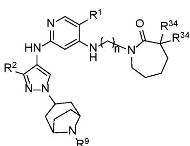
Formula IIIA.23
