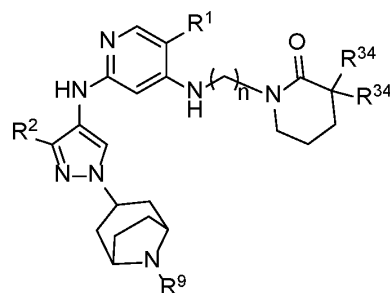
Formula IIIA.24
