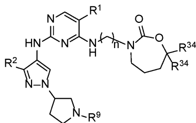
Formula IIA.16
