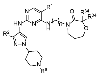
Formula IIA.3
