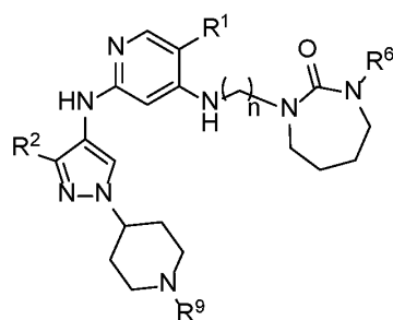
Formula IIIA.8
