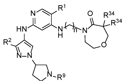
Formula IIIA.10
