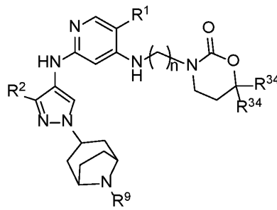
Formula IIIA.20
