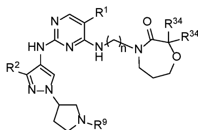
Formula IIA.12
