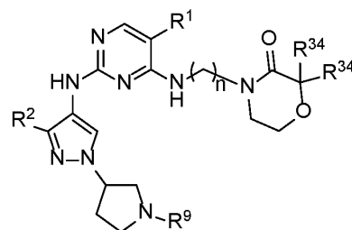
Formula IIA.13
