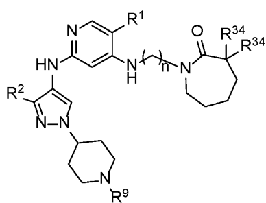
Formula IIIA.5
