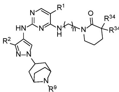
Formula IIA.24
