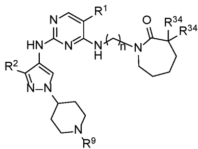
Formula IIA.5
