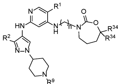
Formula IIIA.7
