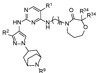
Formula IIA.21
