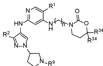
Formula IIIA.11
