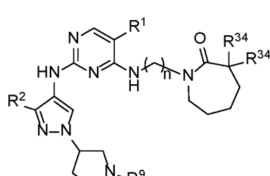
Formula IIA.14
