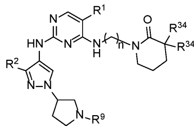
Formula IIA.15
