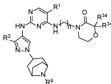
Formula IIA.22
