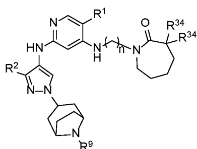
Formula IIIA.23
