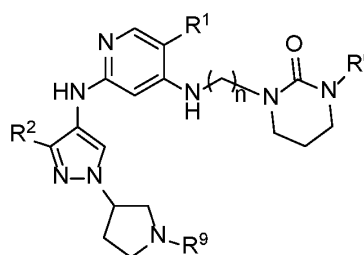
Formula IIIA.18
