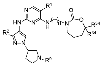
Formula IIA.16
