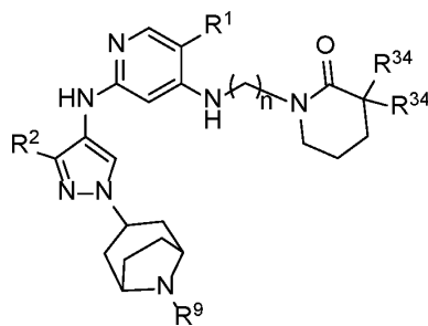
Formula IIIA.24
