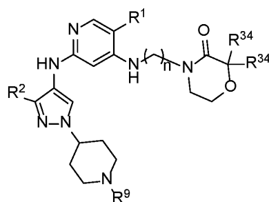
Formula IIIA.4
