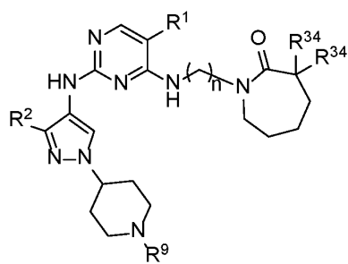
Formula IIA.5
