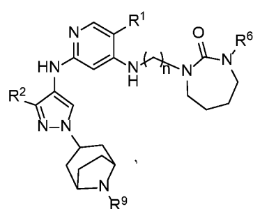
Formula IIIA.26
