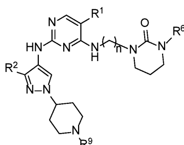
Formula IIA.9
