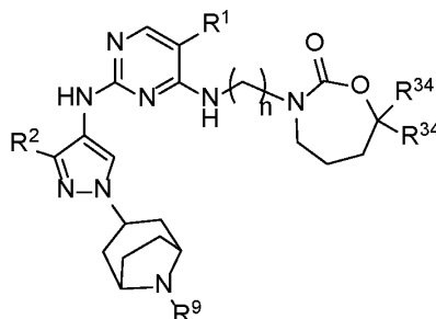
Formula IIA.25
