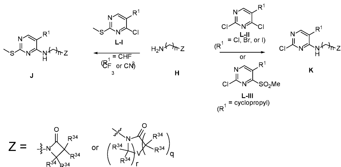
Scheme 21
