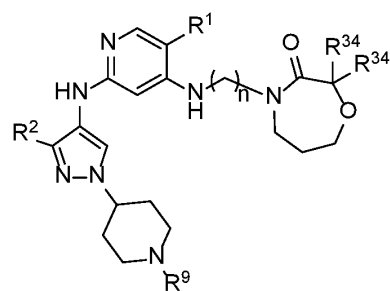
Formula IIIA.3
