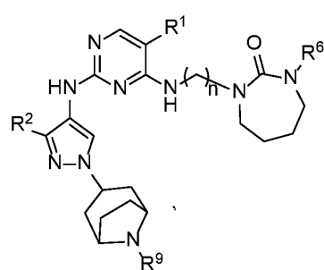
Formula IIA.26
