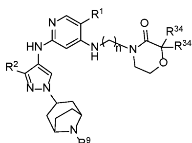
Formula IIIA.22
