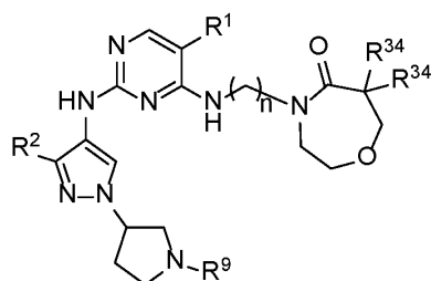
Formula IIA.10
