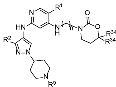
Formula IIIA.2
