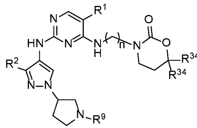
Formula IIA.11
