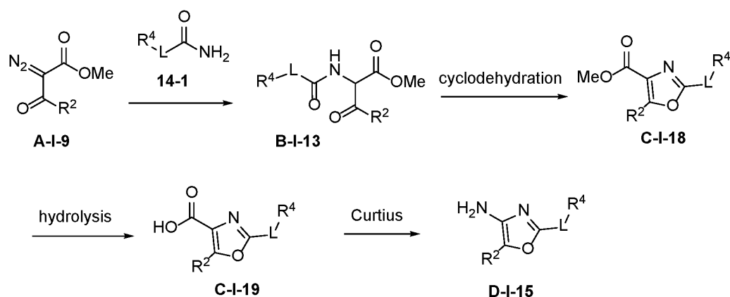
Scheme 13
