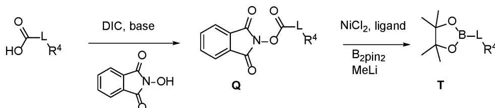
Scheme 16
