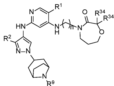
Formula IIIA.21
