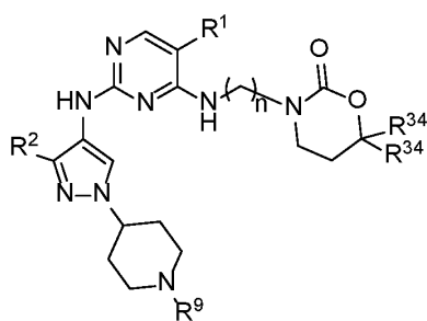
Formula IIA.2
