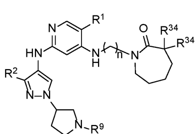
Formula IIIA.14
