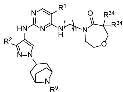
Formula IIA.19
