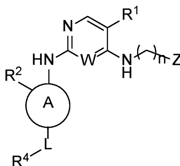
Formula I
