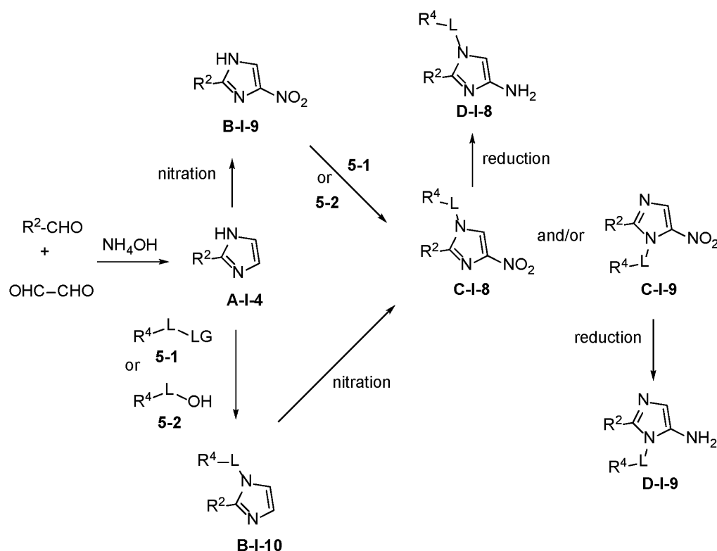
Scheme 7
