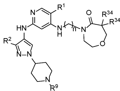
Formula IIIA.1
