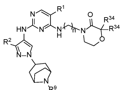
Formula IIA.22
