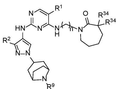
Formula IIA.23
