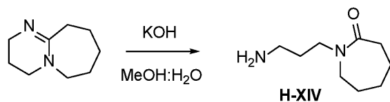
Scheme 20
