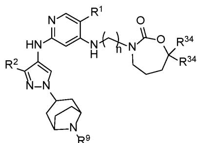
Formula IIIA.25
