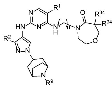
Formula IIA.19
