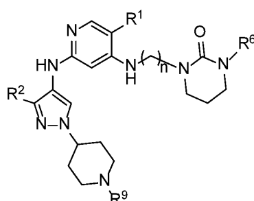
Formula IIIA.9
