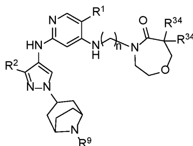
Formula IIIA.19
