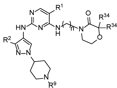
Formula IIA.4
