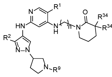
Formula IIIA.15
