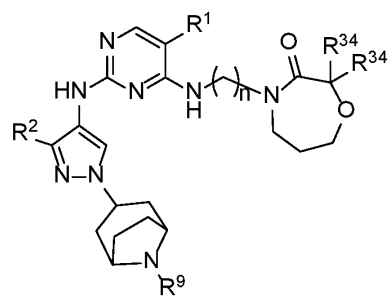
Formula IIA.21
