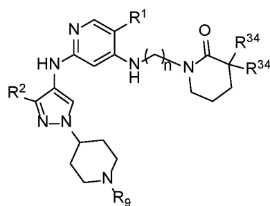
Formula IIIA.6
