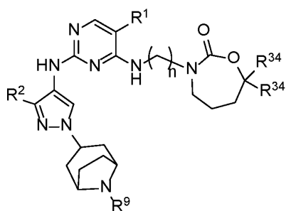
Formula IIA.25
