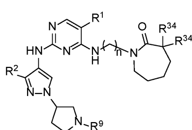
Formula IIA.14
