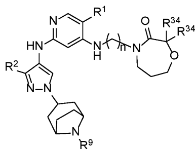
Formula IIIA.21
