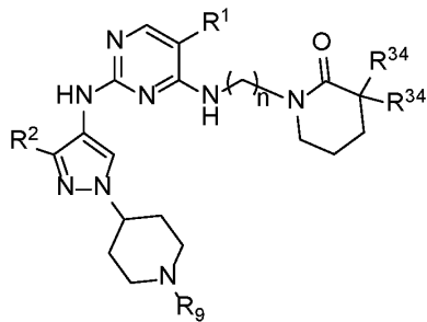
Formula IIA.6
