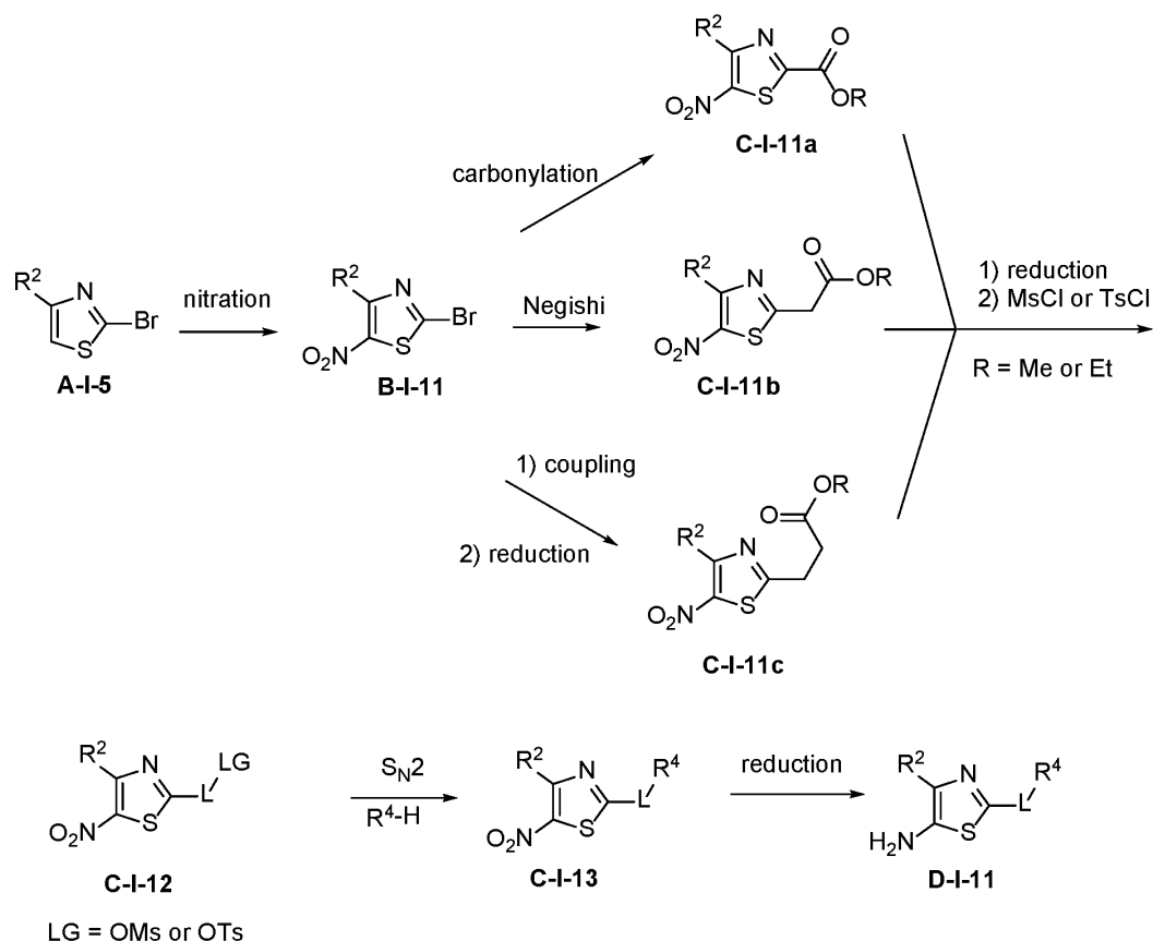
Scheme 9
