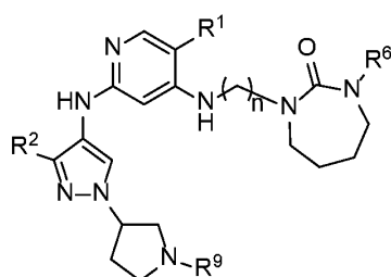
Formula IIIA.17
