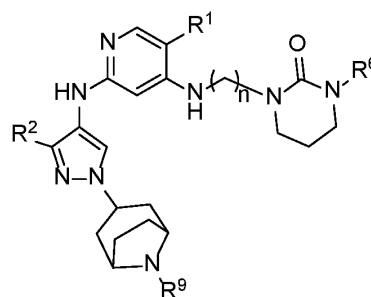
Formula IIIA.27
