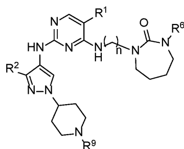
Formula IIA.8
