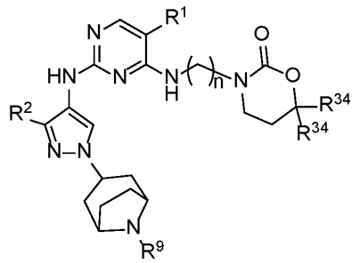
Formula IIA.20
