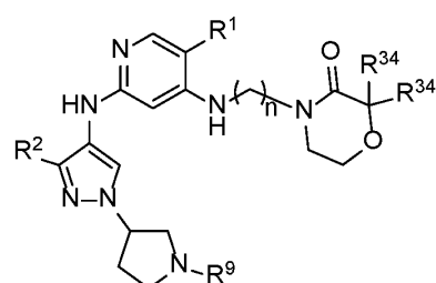
Formula IIIA.13
