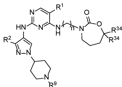
Formula IIA.7
