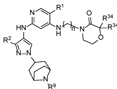
Formula IIIA.22
