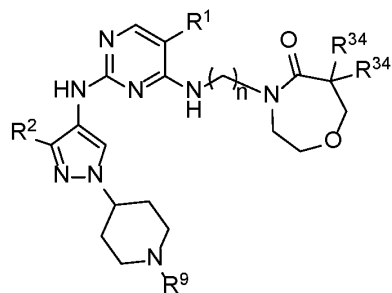
Formula IIA.1
