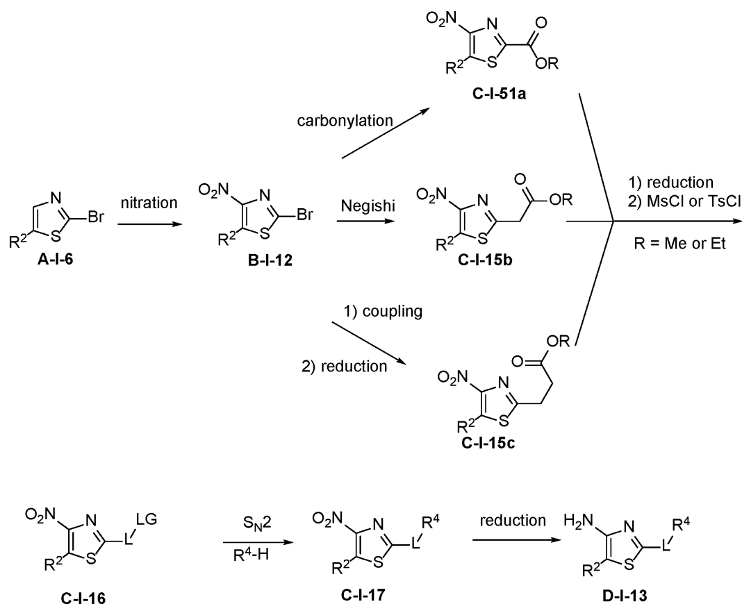
Scheme 11
