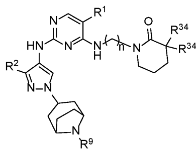
Formula IIA.24
