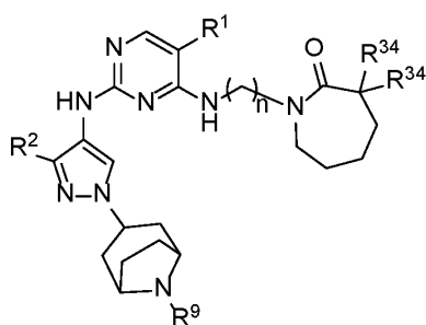
Formula IIA.23
