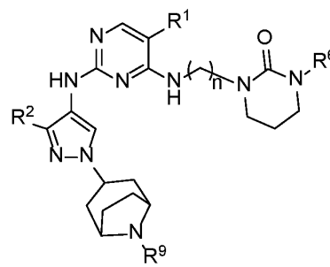
Formula IIA.27
