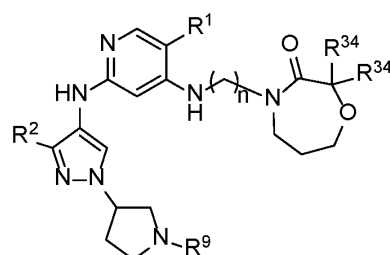
Formula IIIA.12
