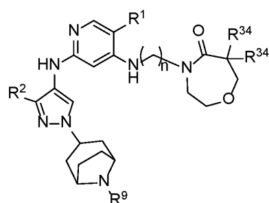
Formula IIIA.19
