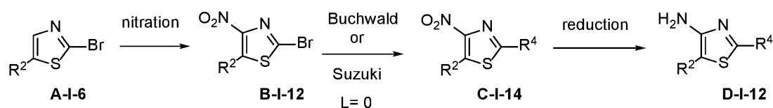
Scheme 10
