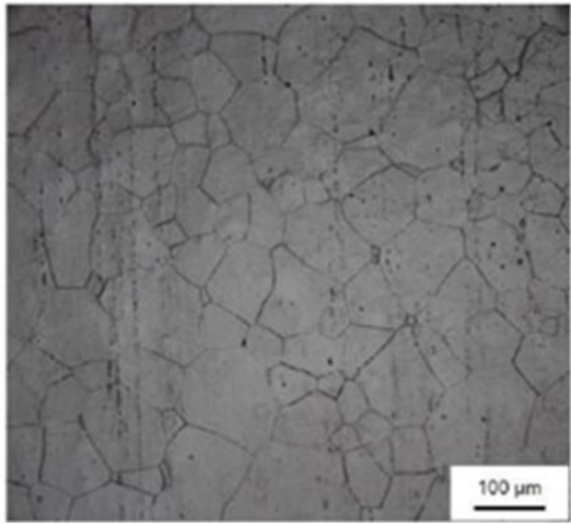
(2) No.1 Annealing material 400^{\circ}\text{C} \times 2 hours
