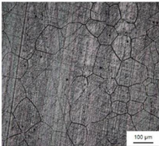
(3) No.1 Annealing material 450^{\circ}\text{C} \times 1 hour
