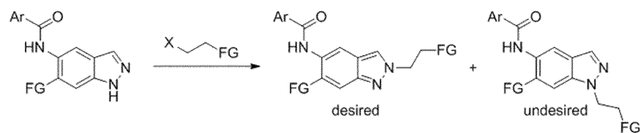
Scheme 1: N-alkylation of 1H-indazoles
