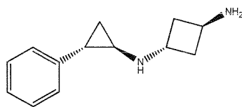
Example 87: (cis)-N1-((1R,2S)-2-phenylcyclopropyl)cyclobutane-1,3-diamine
