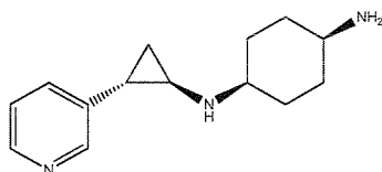
Example 84: (trans)-N1-((1S,2R)-2-(pyridin-3-yl)cyclopropyl)cyclohexane-1,4-diamine
