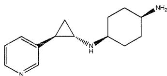
Example 82: (trans)-N1-((1R,2S)-2-(pyridin-3-yl)cyclopropyl)cyclohexane-1,4-diamine
