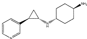
Example 85: (cis)-N1-((1S,2R)-2-phenylcyclopropyl)cyclobutane-1,3-diamine
