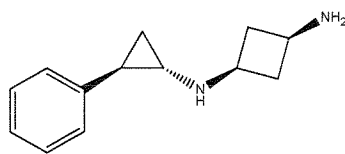
Example 86: (trans)-N1-((1R,2S)-2-phenylcyclopropyl)cyclobutane-1,3-diamine
