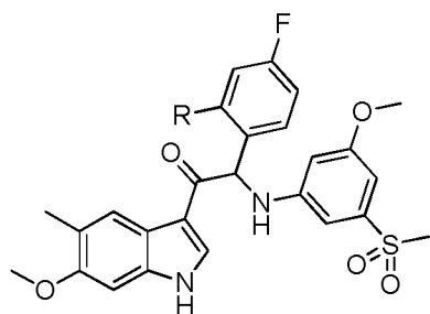
10B (R = OMe)
