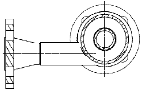
Fig. 5 Section C-C
