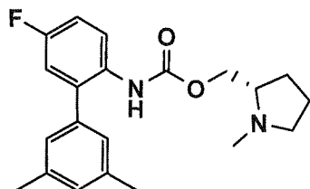
(S)-(1-methylpyrrolidin-2-yl)methyl (2-bromo-4-
