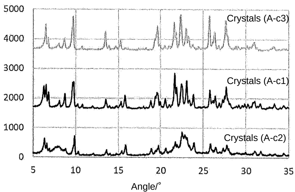
XRD charts of crystals (A) of Examples and Comparative Examples
