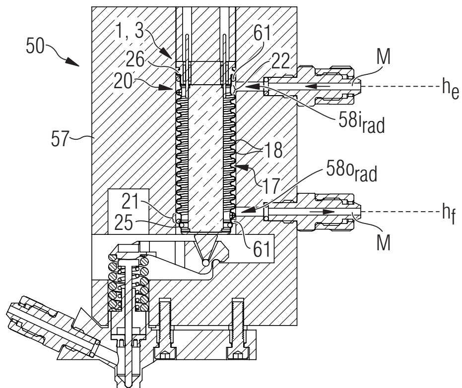
FIG 4 A'-A'
