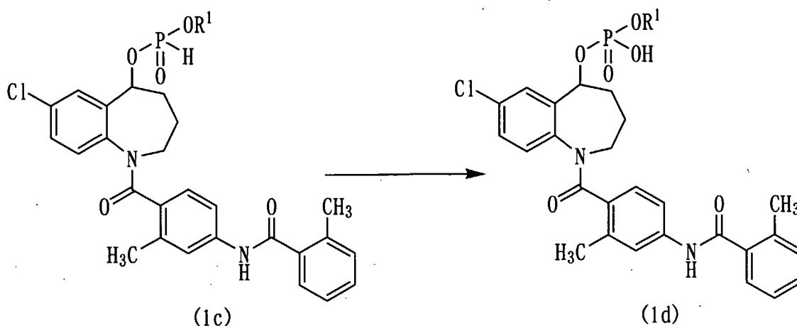
Reaction scheme-4
