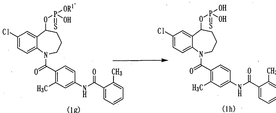
Reaction scheme-7
