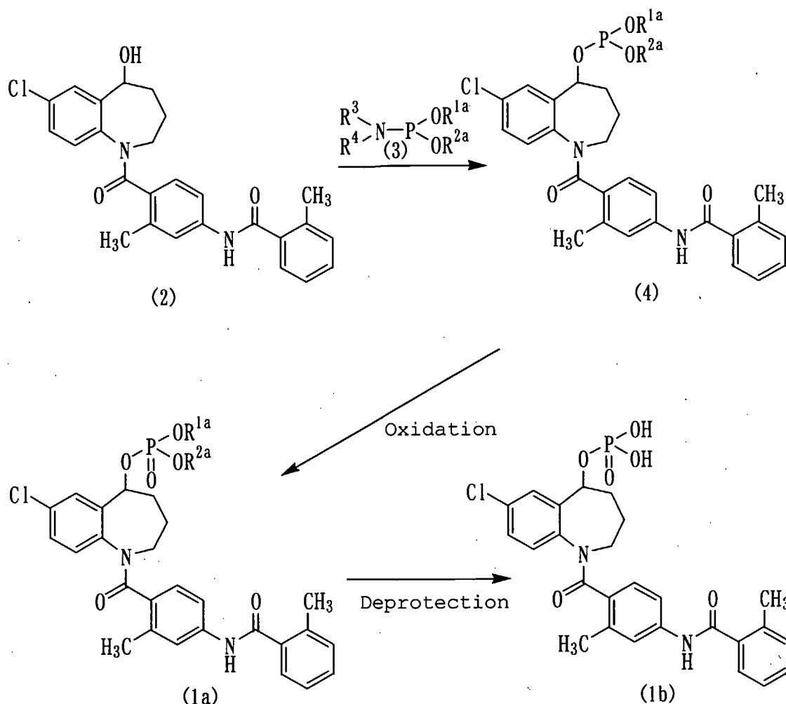
Reaction scheme-1
