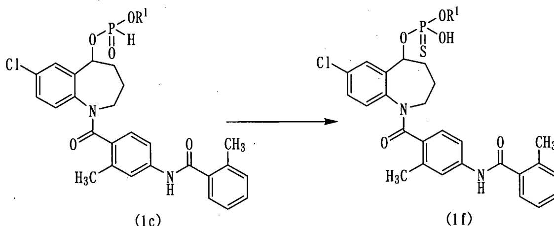
Reaction scheme-6
