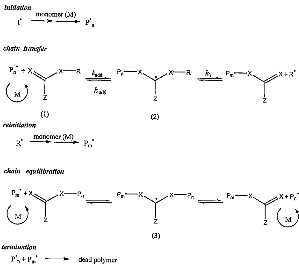
Scheme 1. Proposed mechanism of RAFT polymerisation
