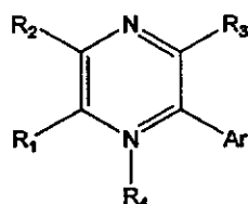
Formula IA
