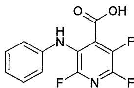
2,3,6-Trifluoro-5-phenylamino-isonicotinic acid,
