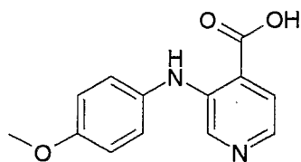
3-(4-Methoxy-phenylamino)-isonicotinic acid,
