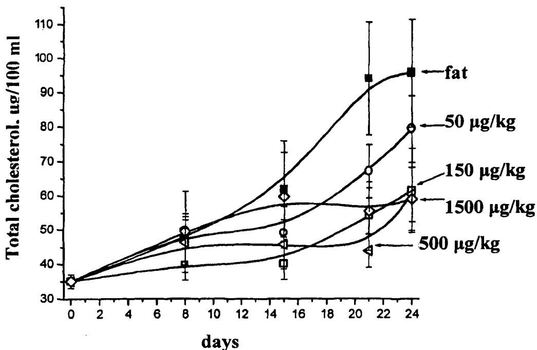
Fig.1. Change in serum total cholesterol level as effected by fat loading and different doses (50-1,500 \mu\text{g/kg} ) of compound IV. Thin vertical lines indicate standard deviation from the mean value.
